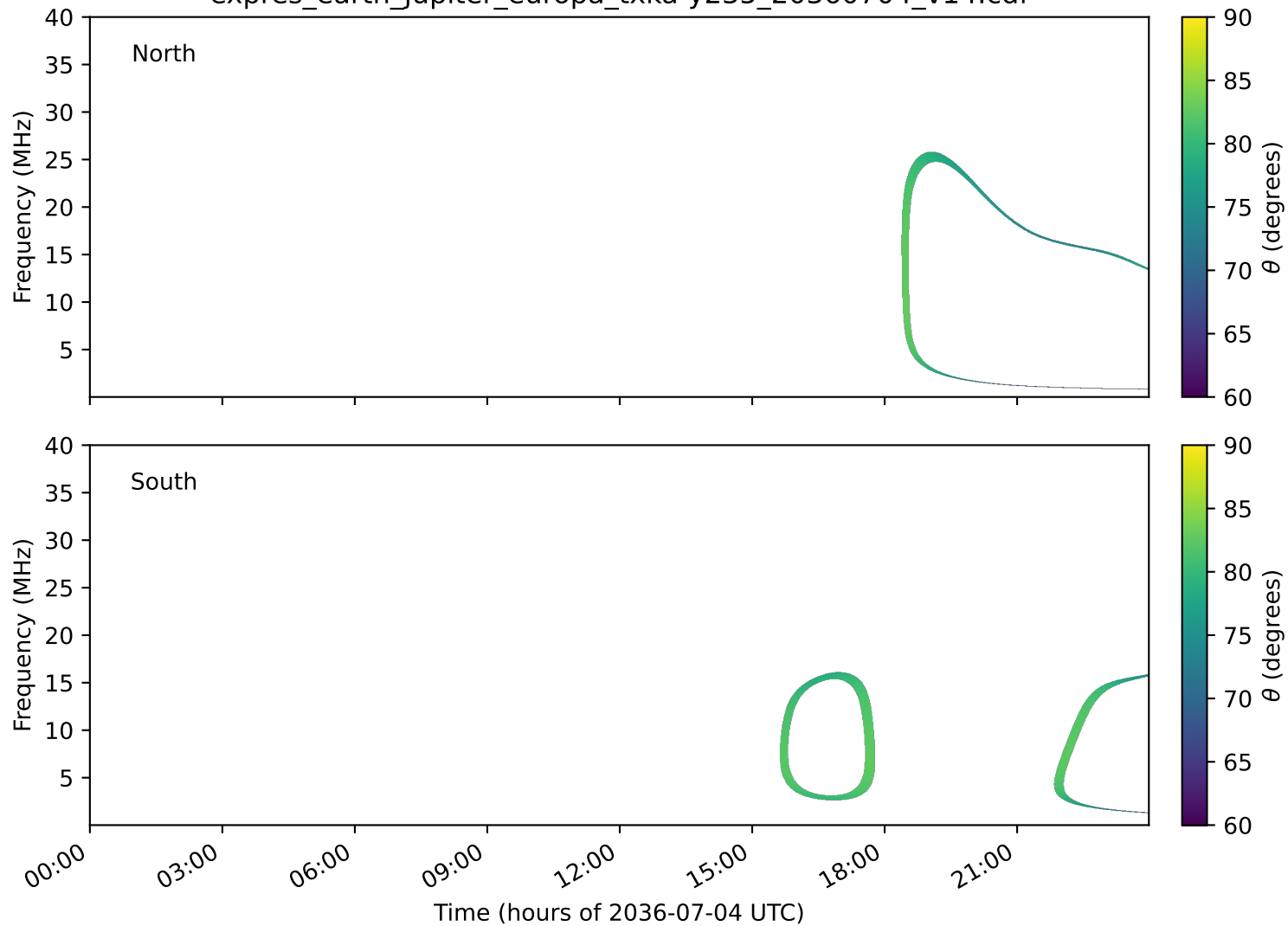
expres_earth_jupiter_europa_txka-y235_20360704_v14.cdf
