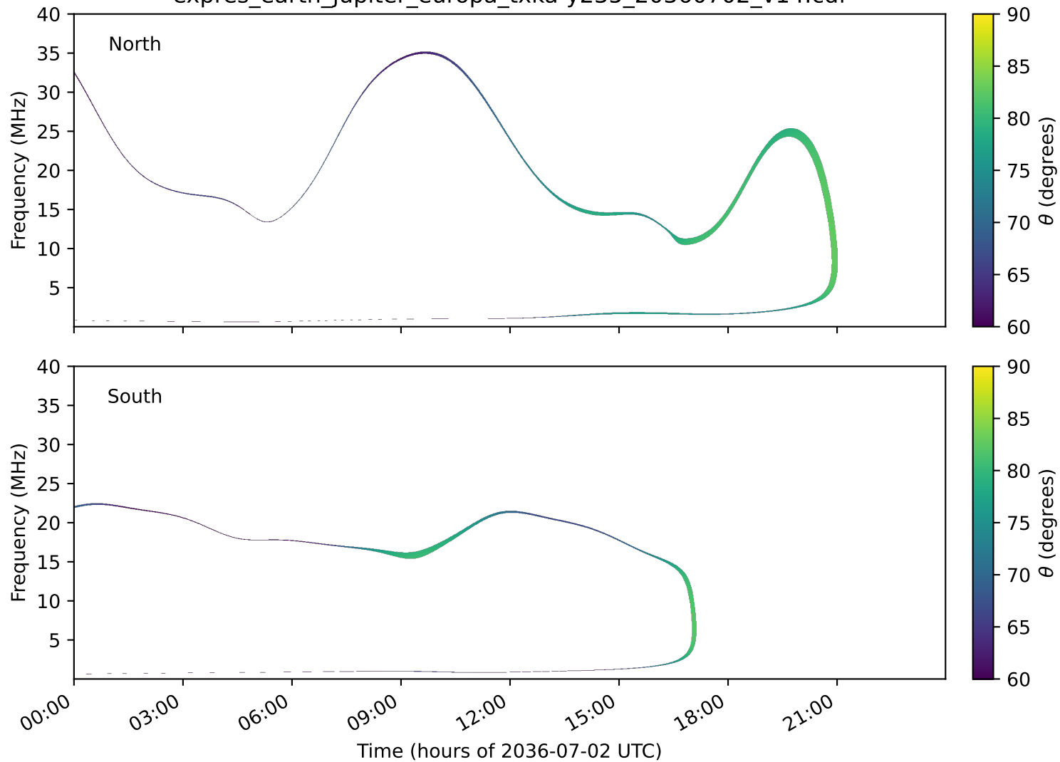
expres_earth_jupiter_europa_txka-y235_20360702_v14.cdf
