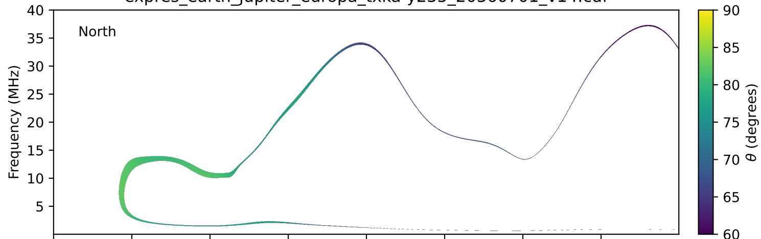
expres_earth_jupiter_europa_txka-y235_20360701_v14.cdf
