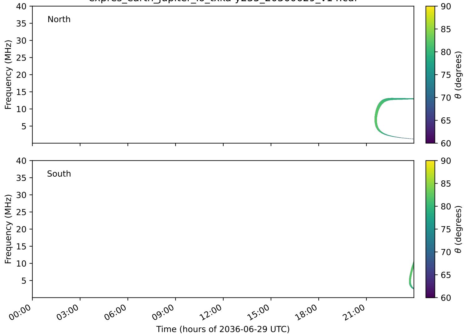
expres_earth_jupiter_io_txka-y235_20360629_v14.cdf
