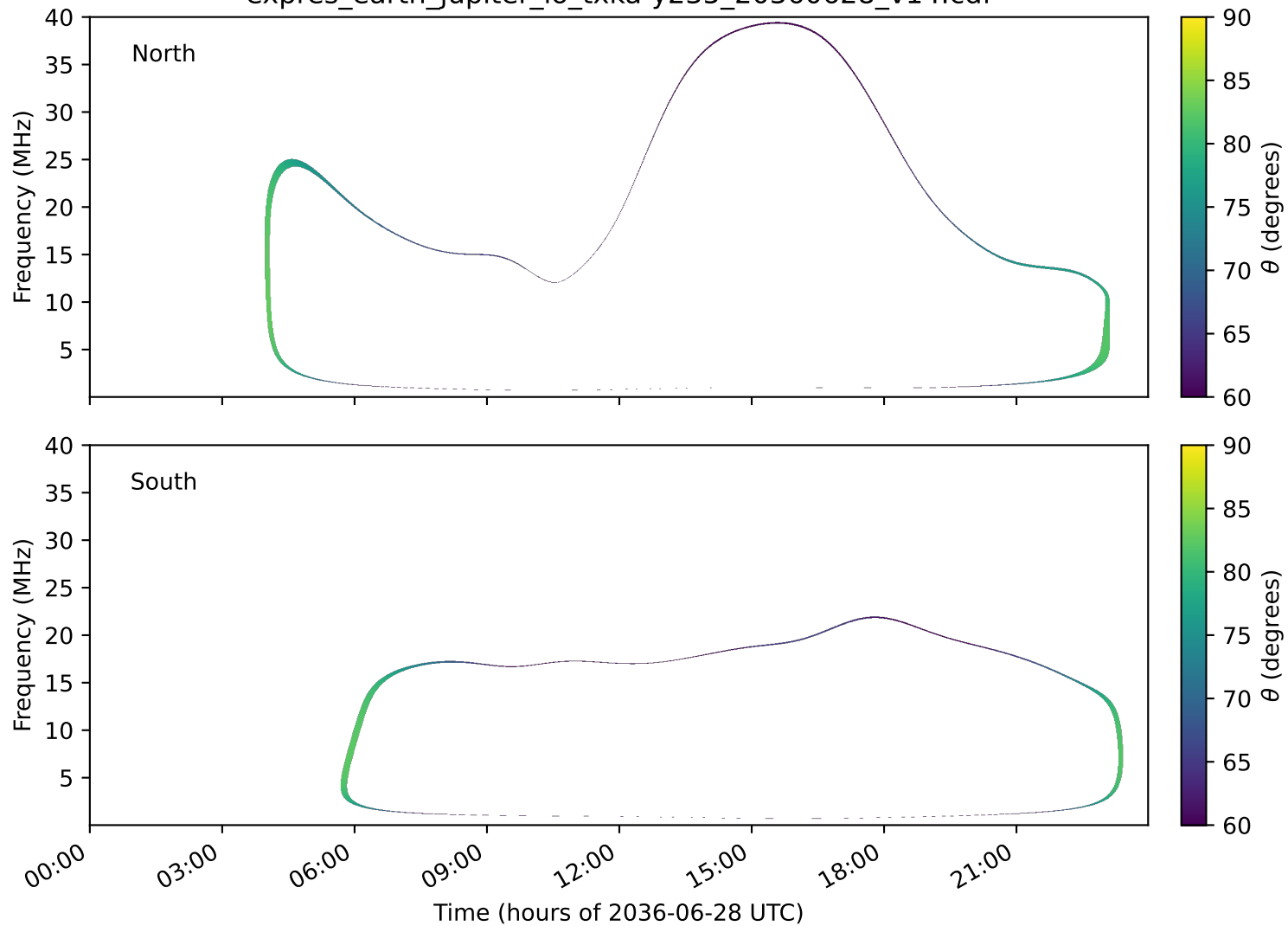
expres_earth_jupiter_io_txka-y235_20360628_v14.cdf
