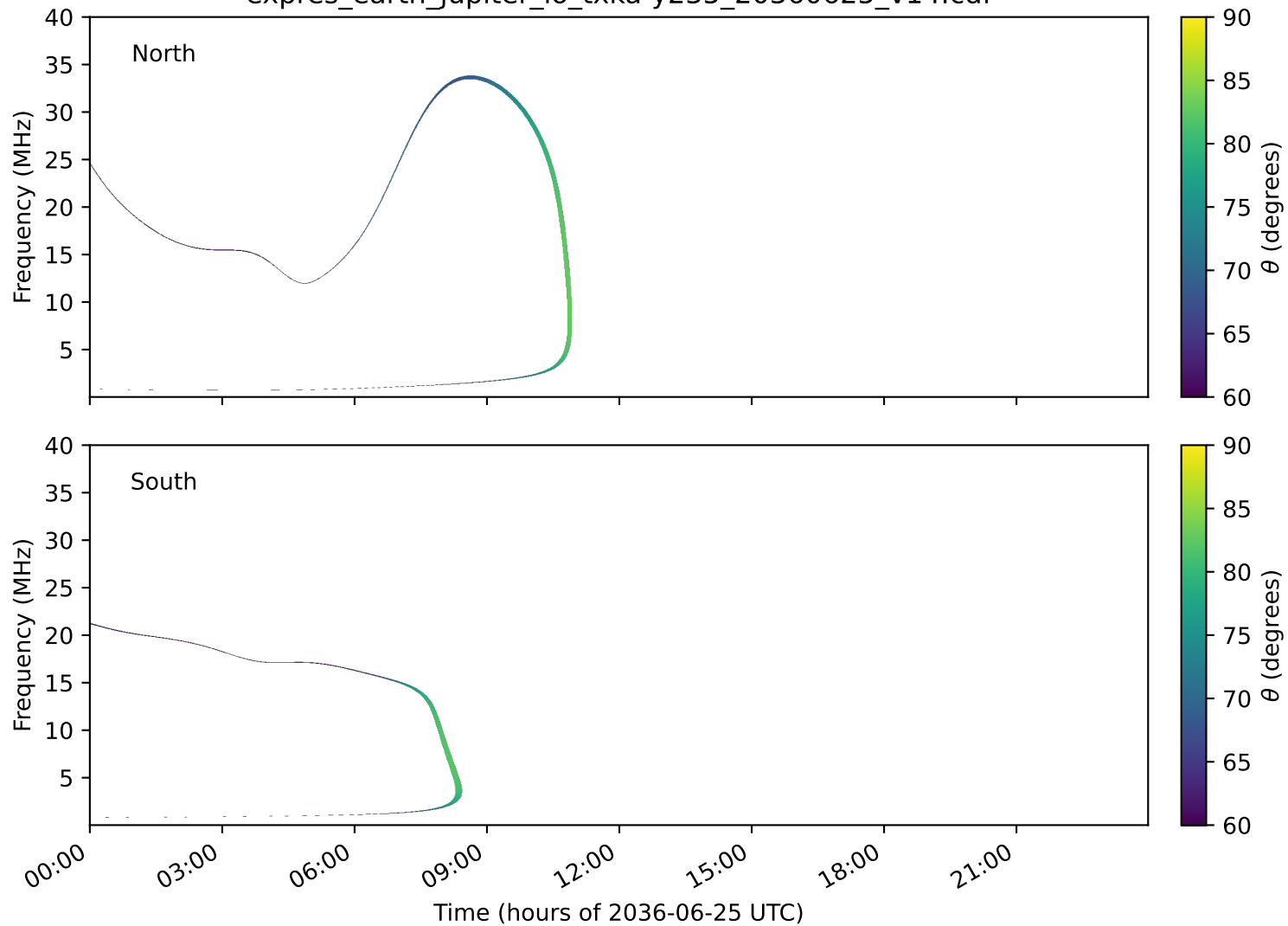
expres_earth_jupiter_io_txka-y235_20360625_v14.cdf
