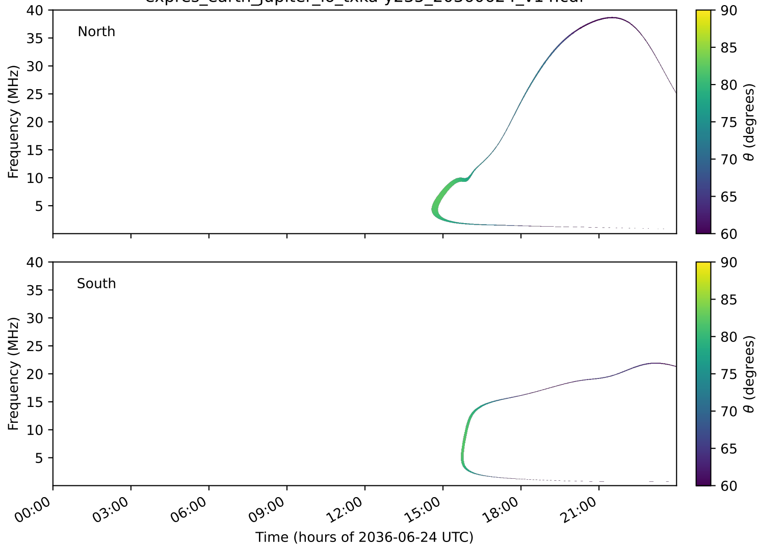
expres_earth_jupiter_io_txka-y235_20360624_v14.cdf
