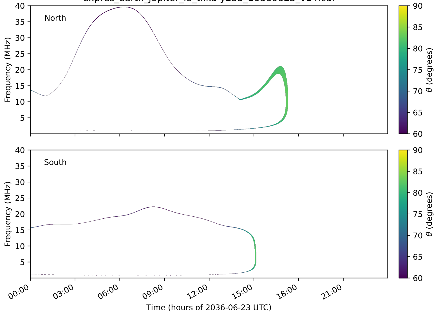
expres_earth_jupiter_io_txka-y235_20360623_v14.cdf
