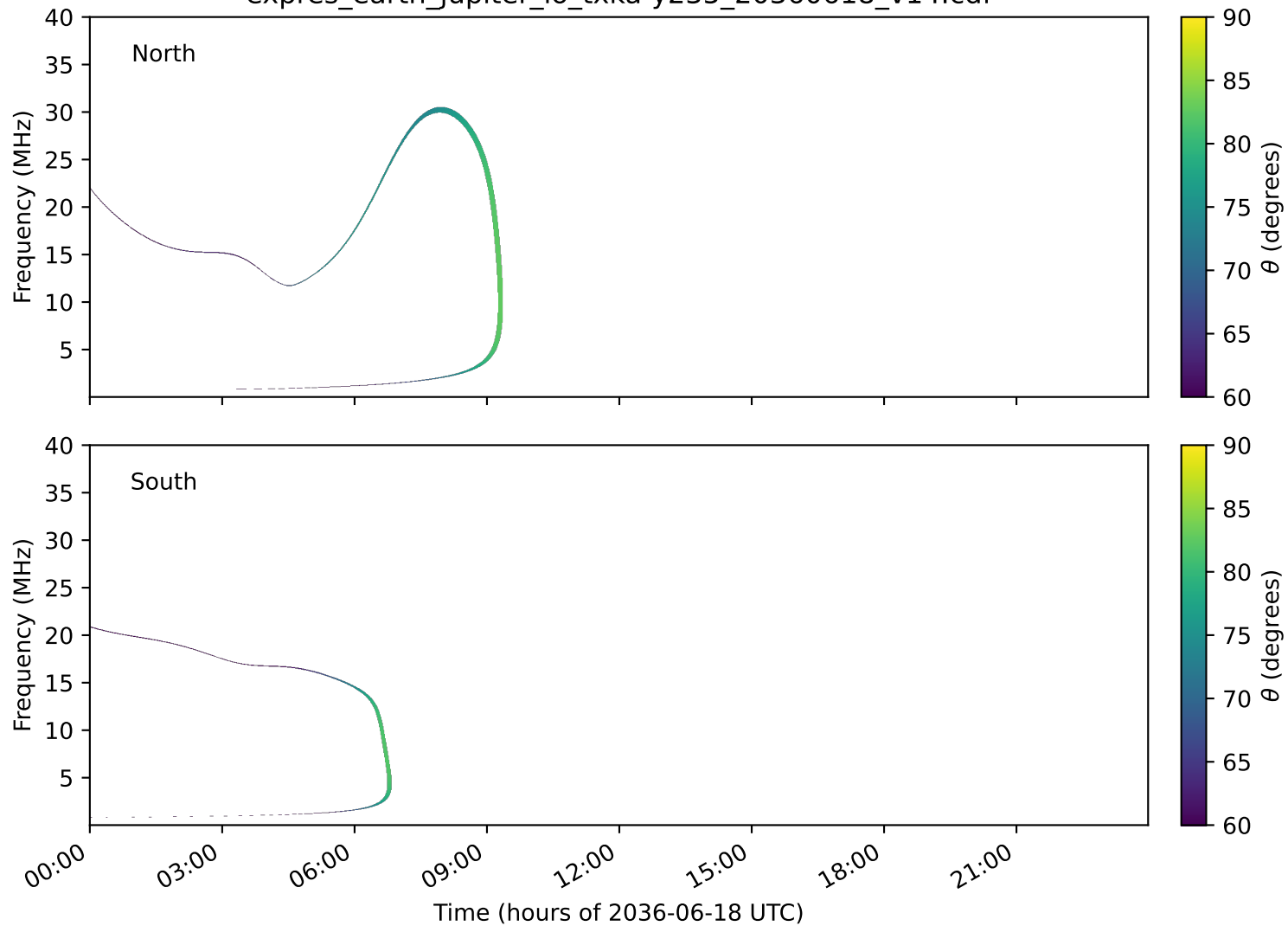
expres_earth_jupiter_io_txka-y235_20360618_v14.cdf
