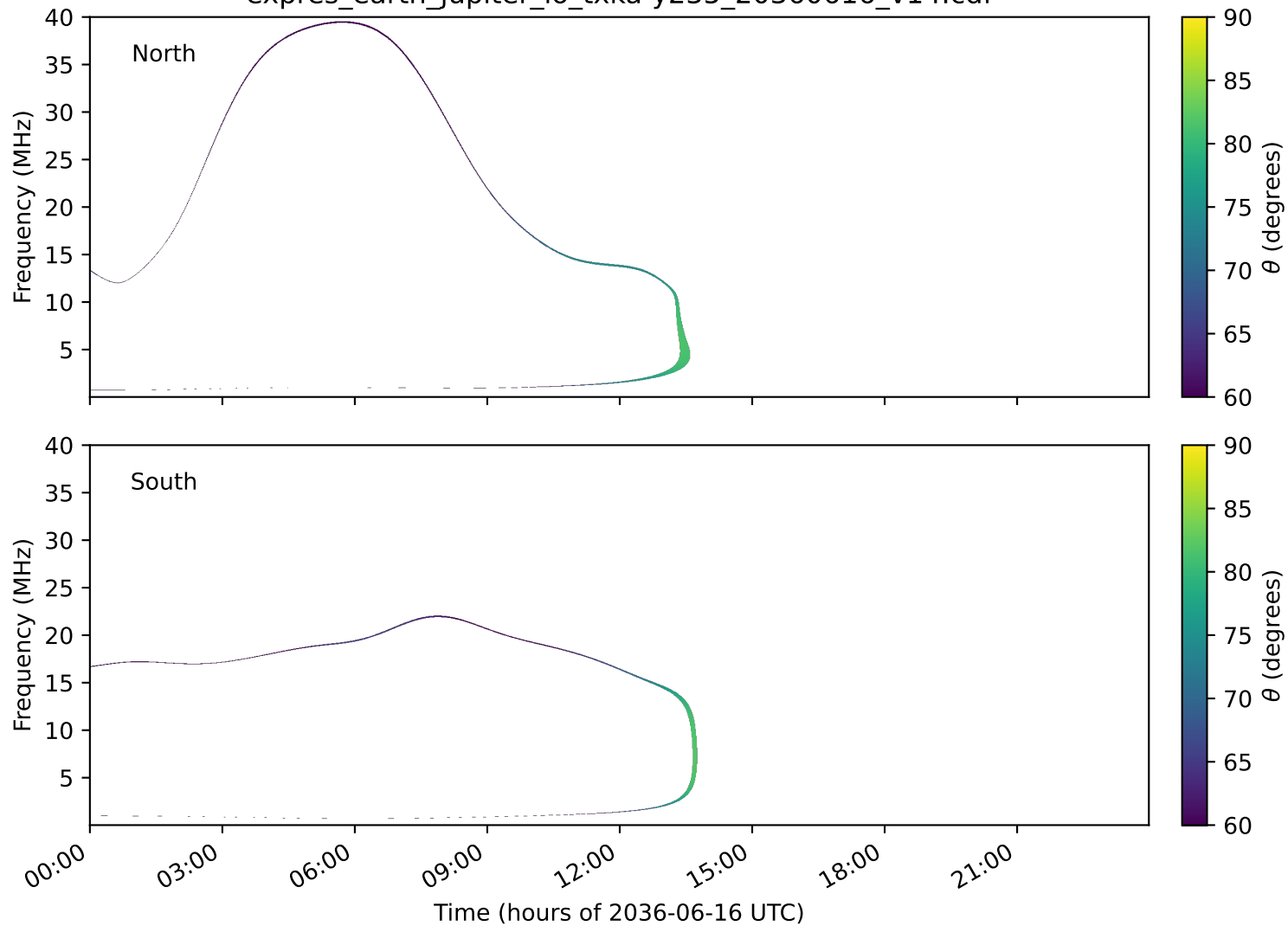
expres_earth_jupiter_io_txka-y235_20360616_v14.cdf
