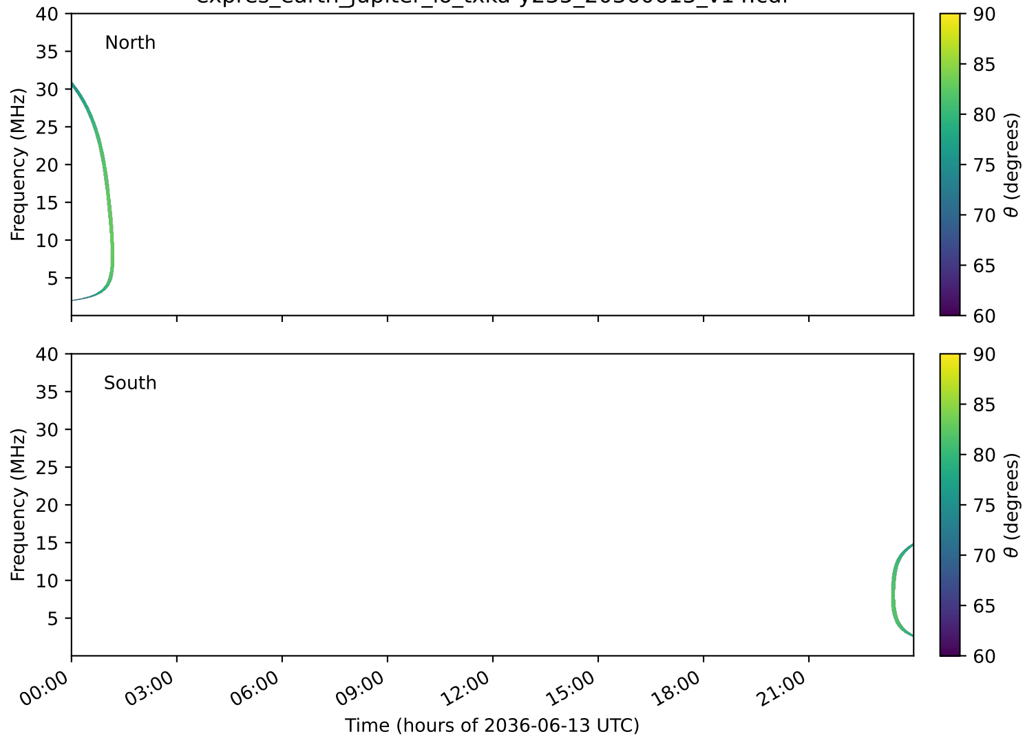
expres_earth_jupiter_io_txka-y235_20360613_v14.cdf
