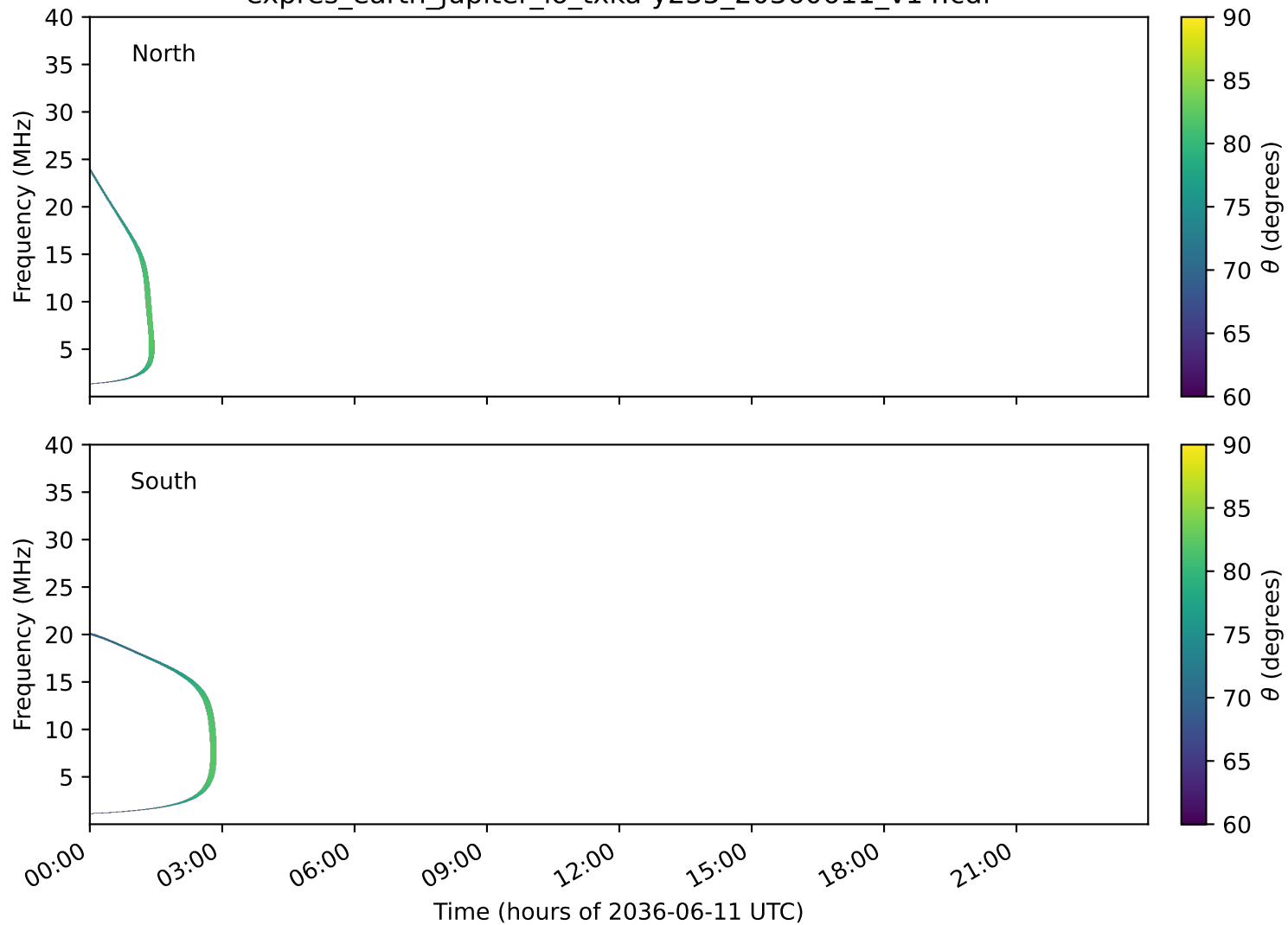
expres_earth_jupiter_io_txka-y235_20360611_v14.cdf
