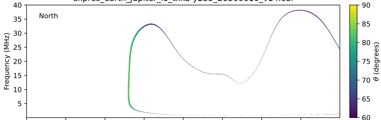
expres_earth_jupiter_io_txka-y235_20360610_v14.cdf
