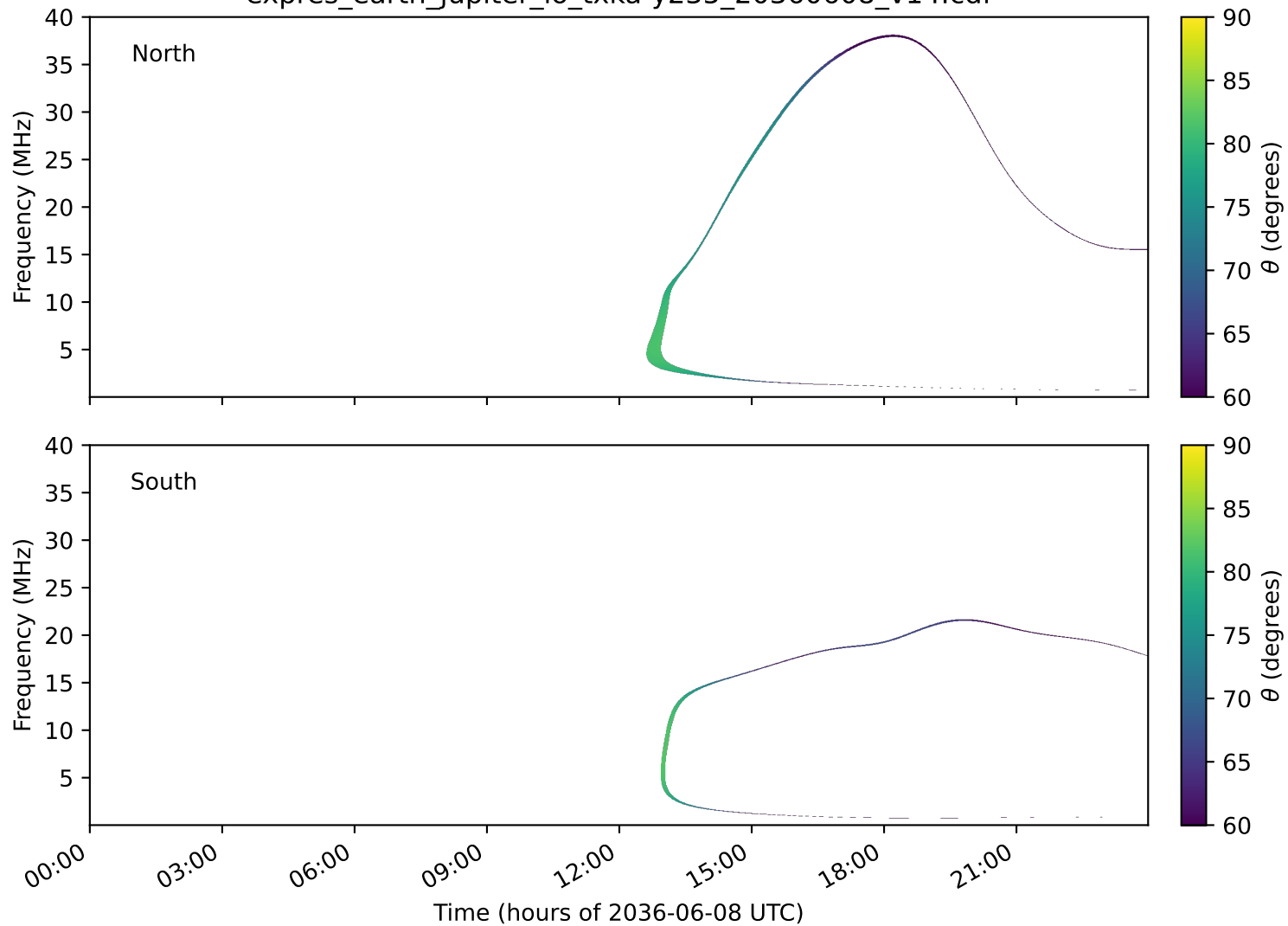
expres_earth_jupiter_io_txka-y235_20360608_v14.cdf
