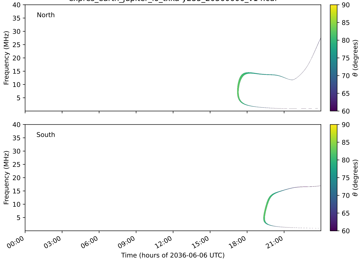
expres_earth_jupiter_io_txka-y235_20360606_v14.cdf
