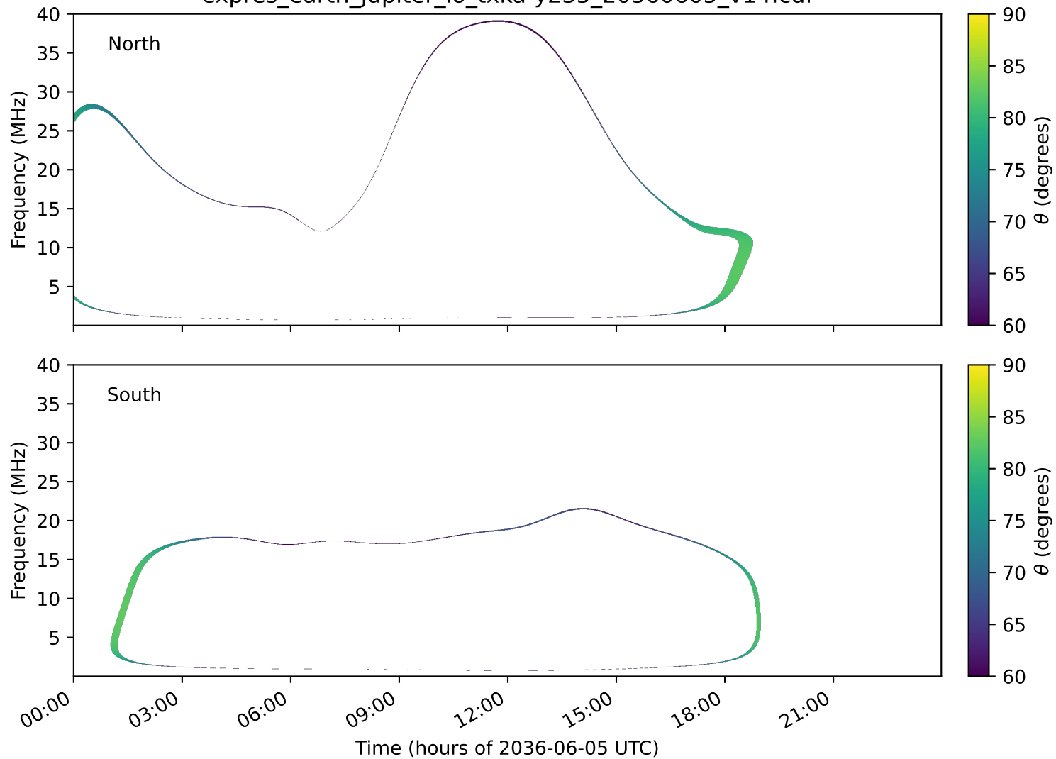
expres_earth_jupiter_io_txka-y235_20360605_v14.cdf
