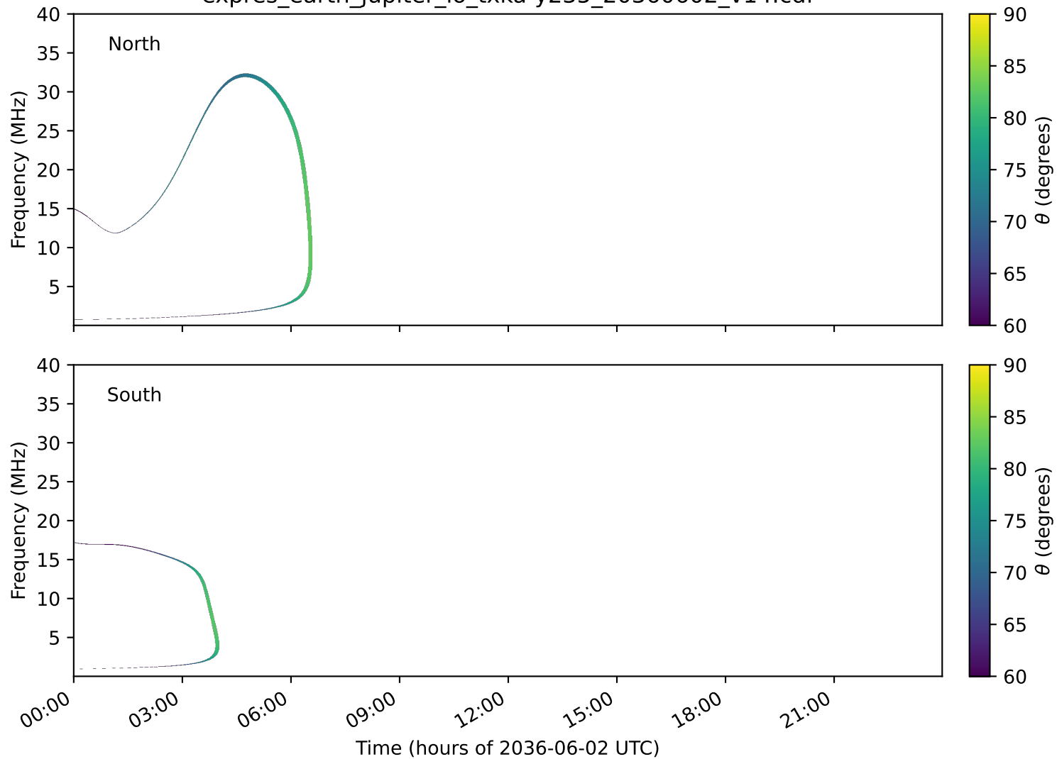
expres_earth_jupiter_io_txka-y235_20360602_v14.cdf
