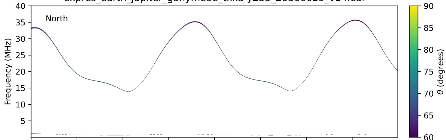
expres_earth_jupiter_ganymede_txka-y235_20360629_v14.cdf
