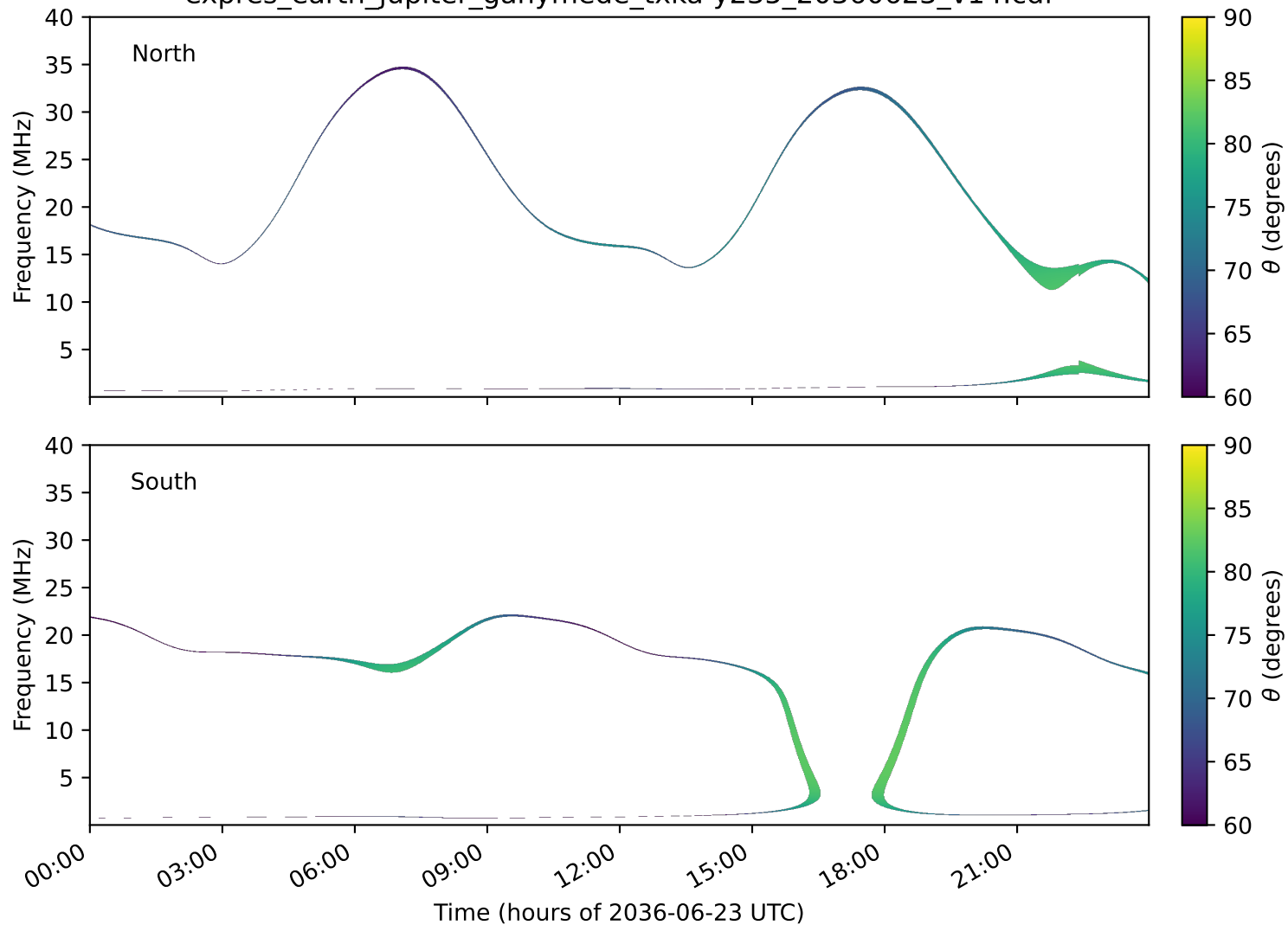
expres_earth_jupiter_ganymede_txka-y235_20360623_v14.cdf
