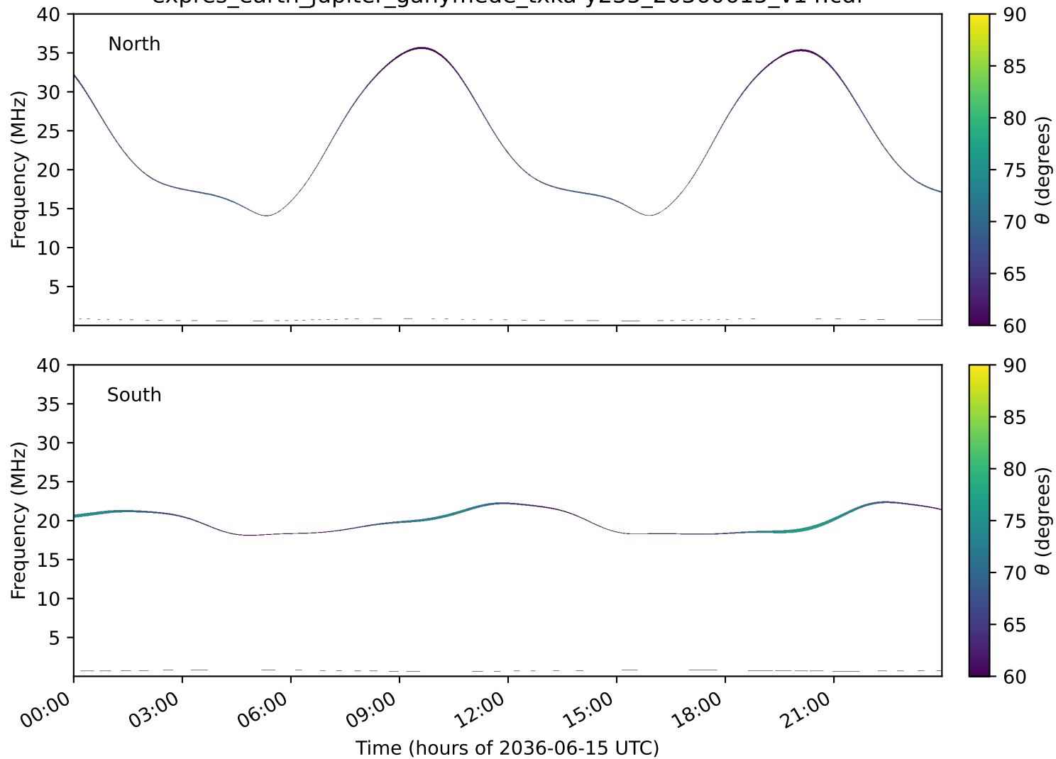
expres_earth_jupiter_ganymede_txka-y235_20360615_v14.cdf
