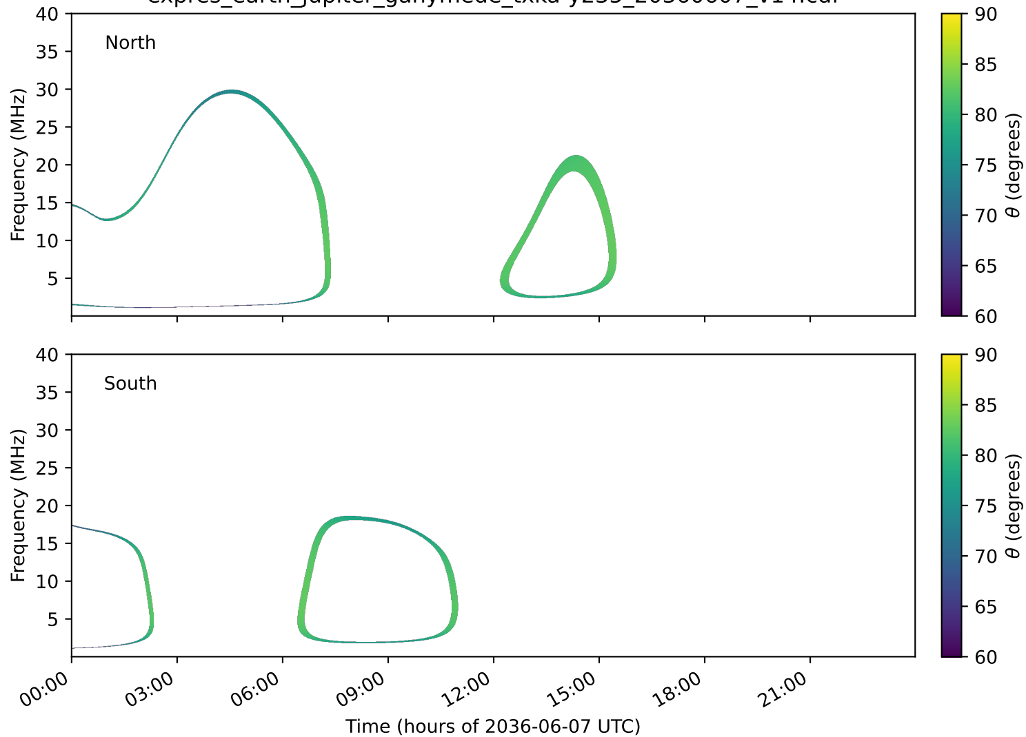
expres_earth_jupiter_ganymede_txka-y235_20360607_v14.cdf
