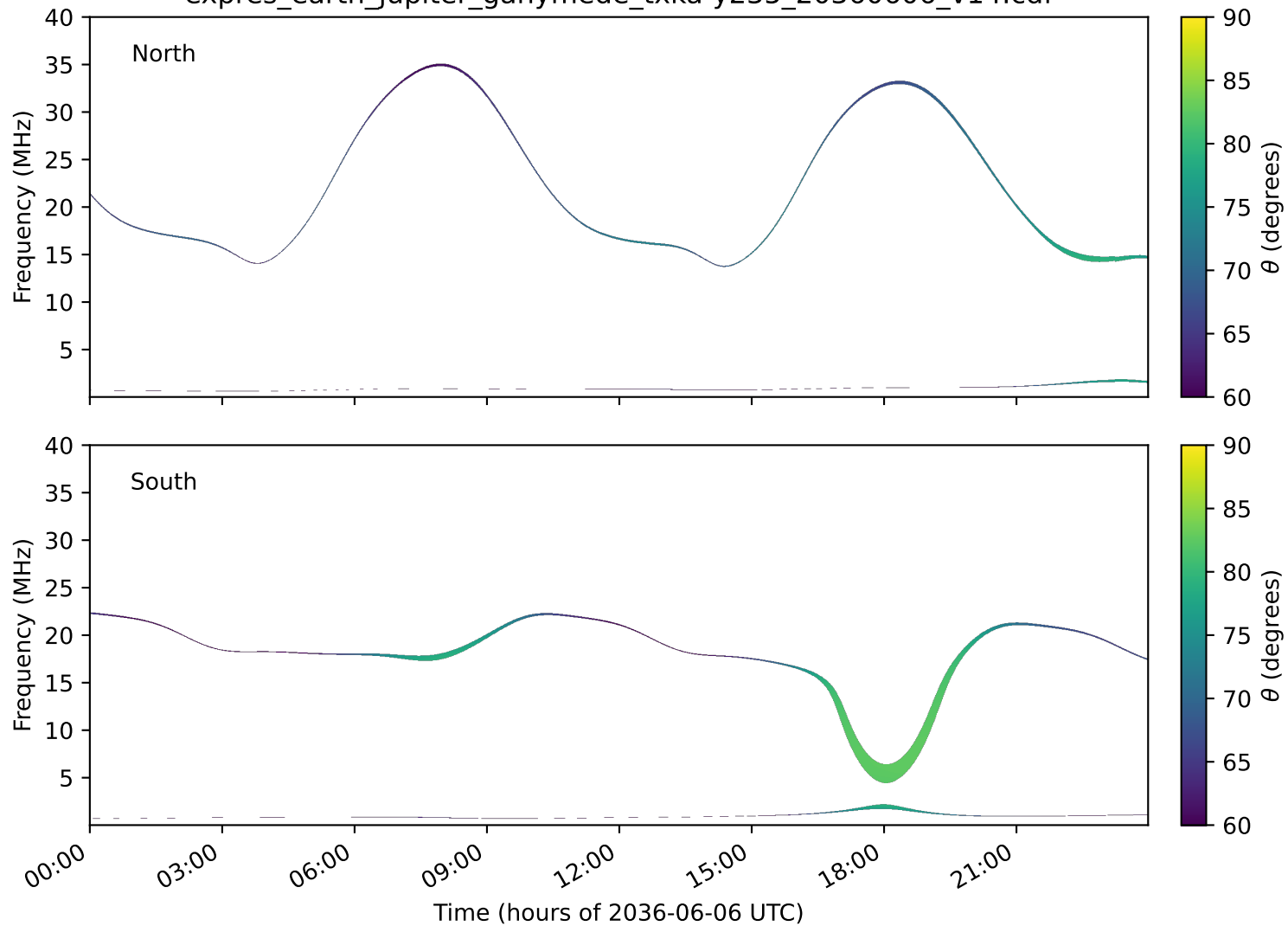
expres_earth_jupiter_ganymede_txka-y235_20360606_v14.cdf
