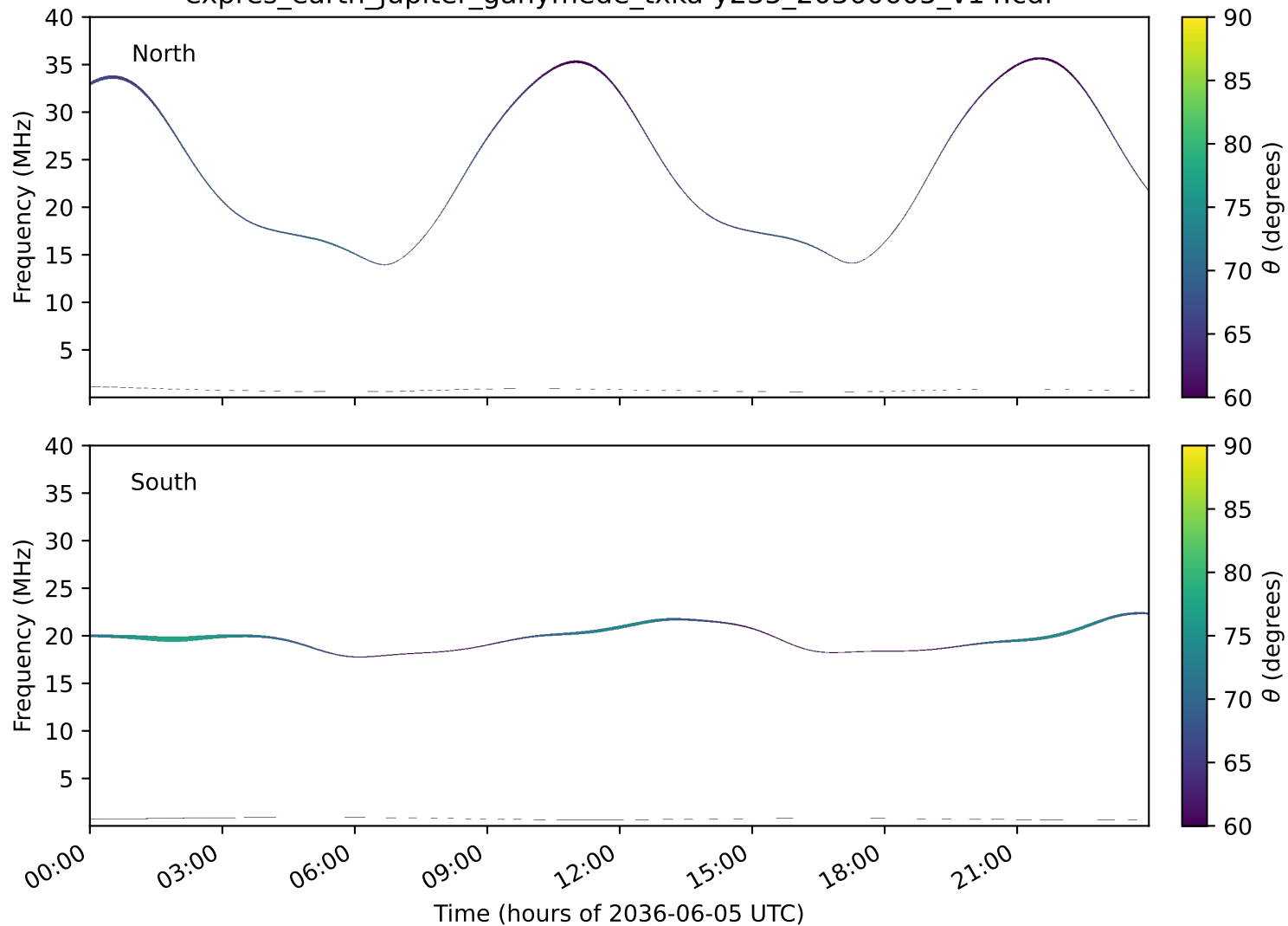
expres_earth_jupiter_ganymede_txka-y235_20360605_v14.cdf
