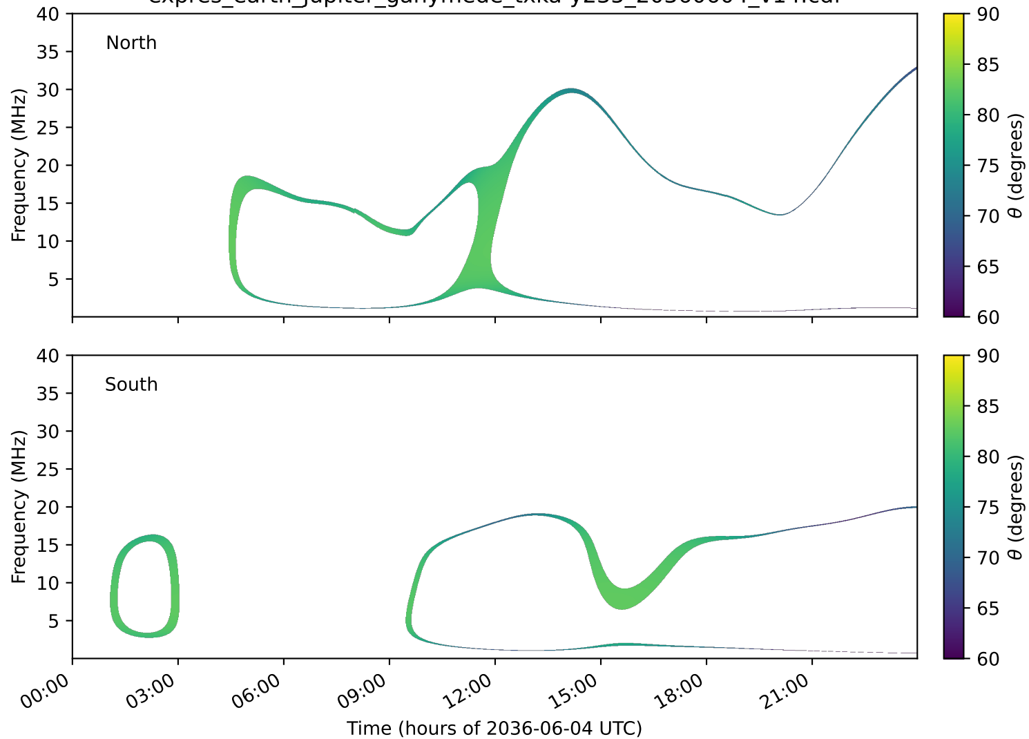
expres_earth_jupiter_ganymede_txka-y235_20360604_v14.cdf
