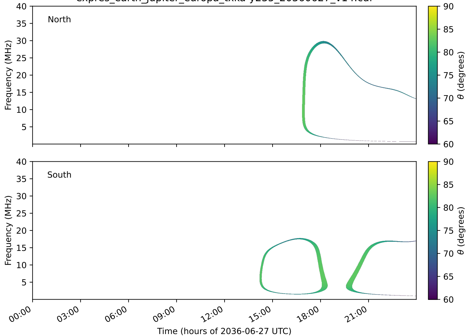
expres_earth_jupiter_europa_txka-y235_20360627_v14.cdf
