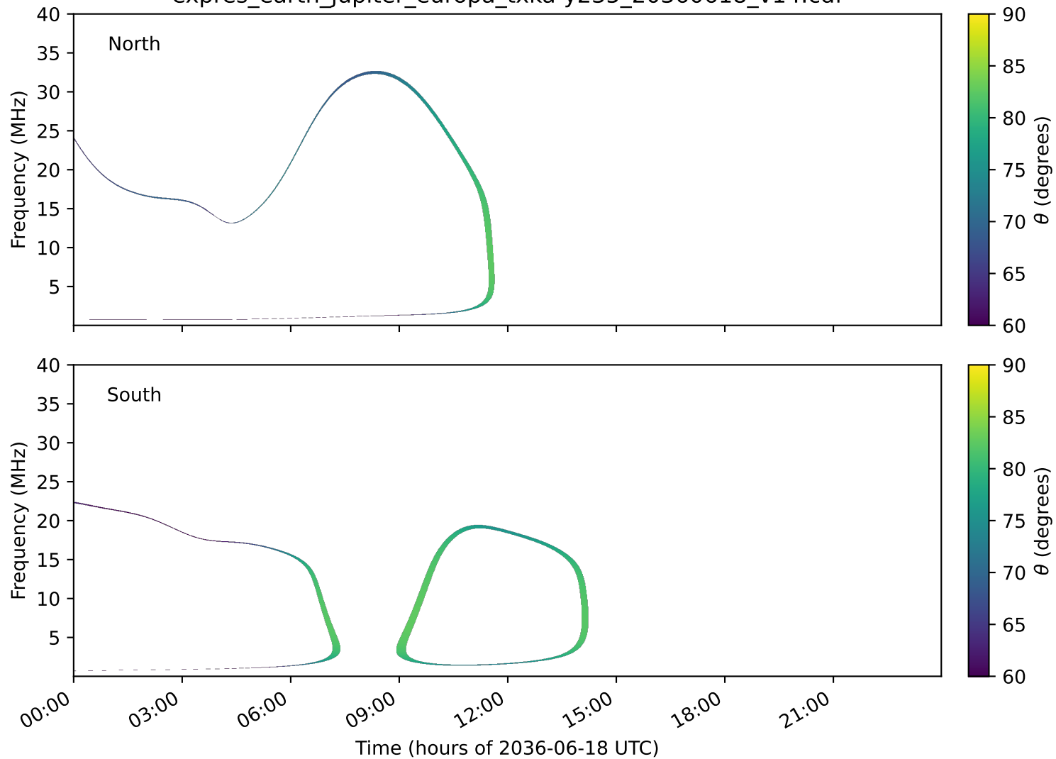
expres_earth_jupiter_europa_txka-y235_20360618_v14.cdf
