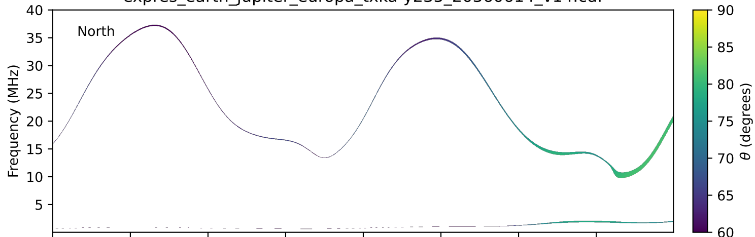
expres_earth_jupiter_europa_txka-y235_20360614_v14.cdf
