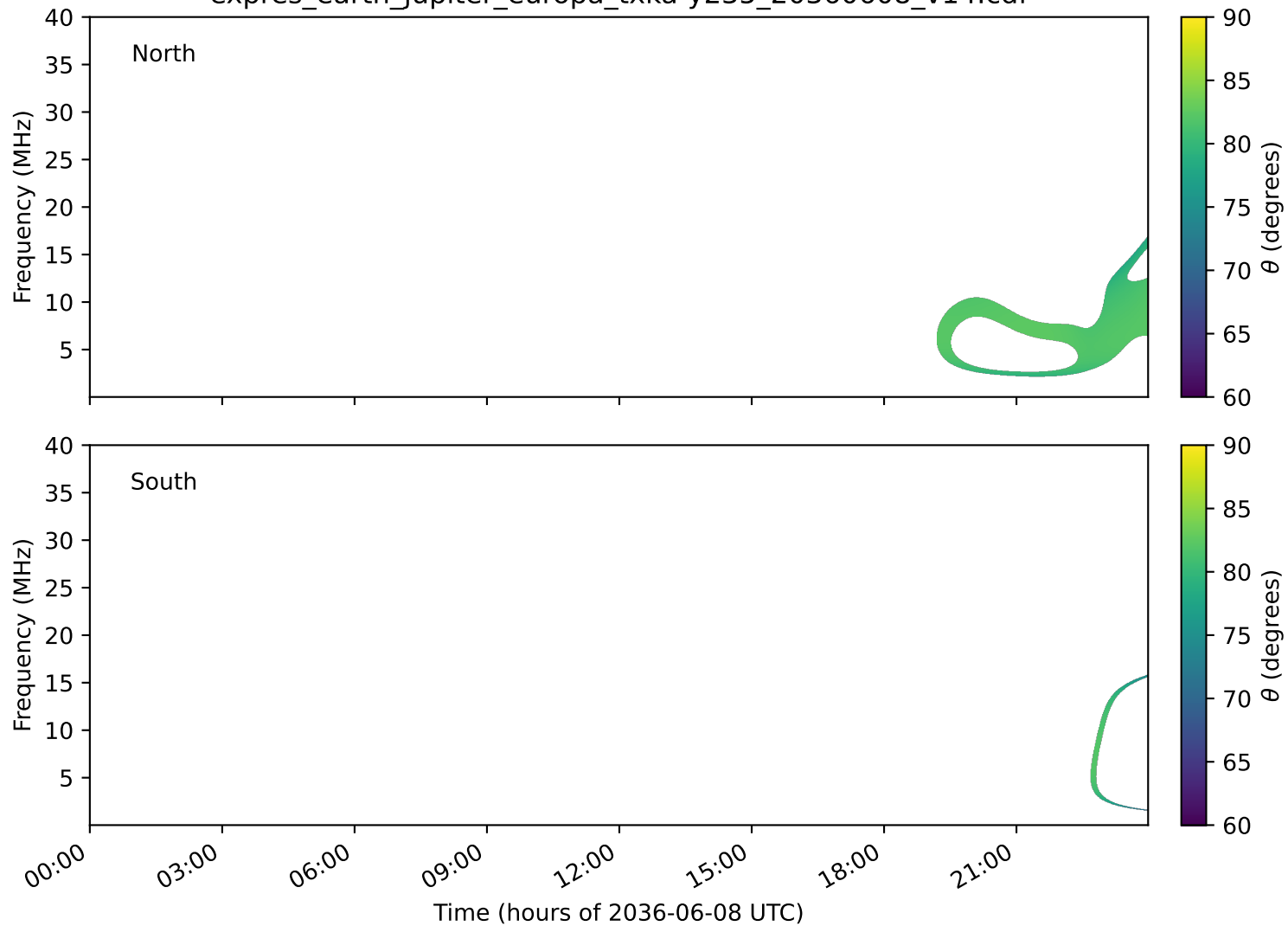
expres_earth_jupiter_europa_txka-y235_20360608_v14.cdf
