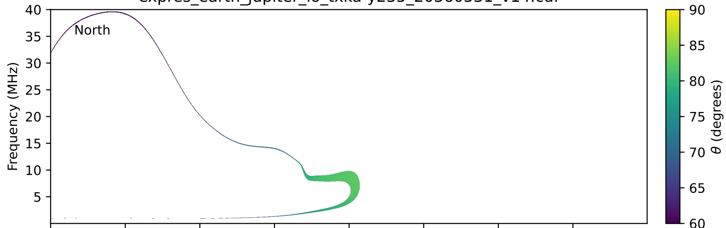
expres_earth_jupiter_io_txka-y235_20360531_v14.cdf
