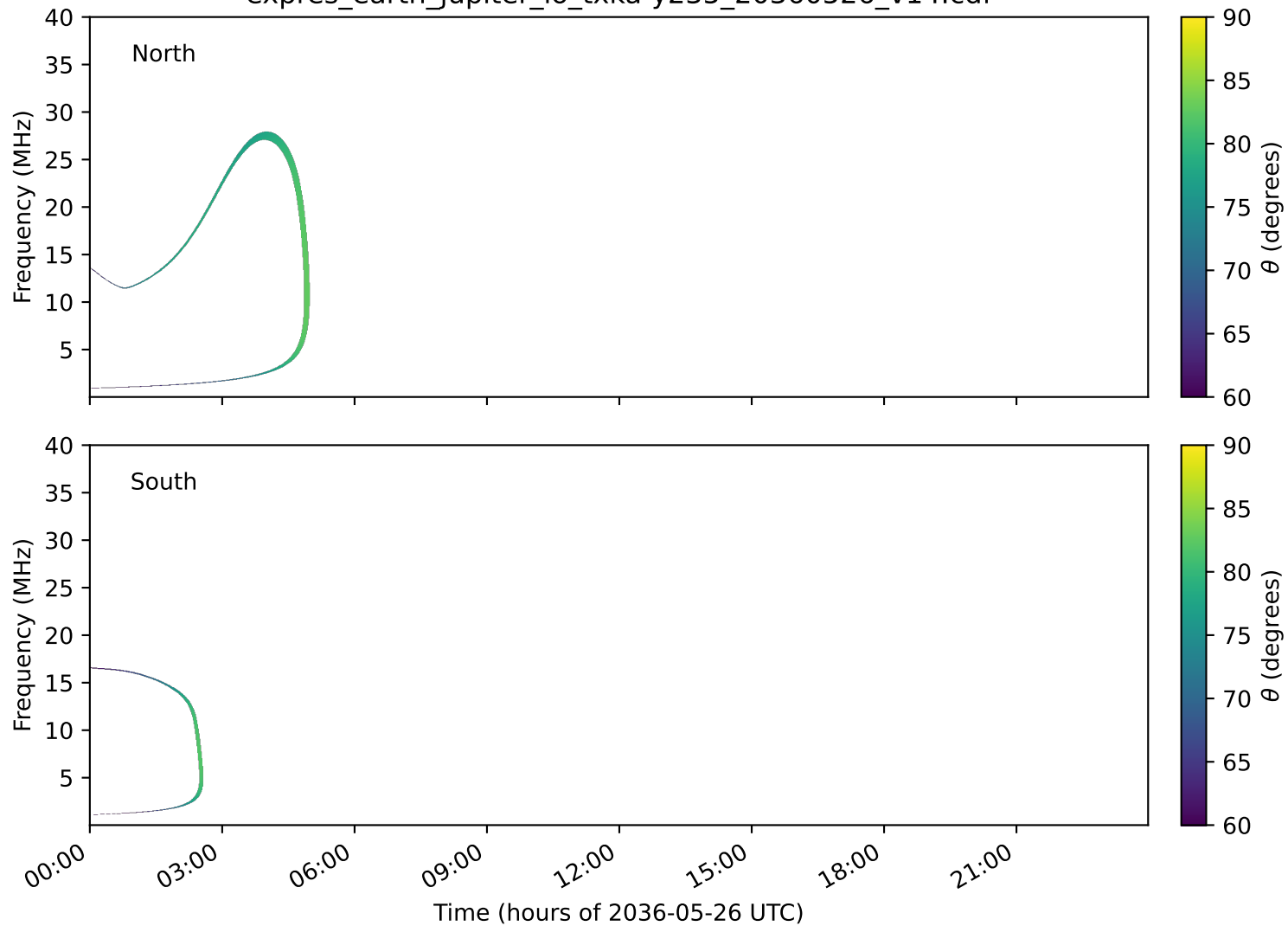
expres_earth_jupiter_io_txka-y235_20360526_v14.cdf
