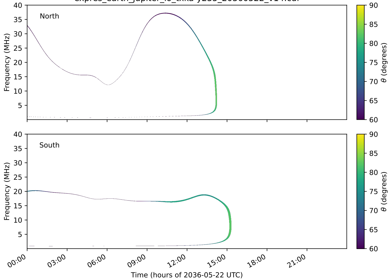
expres_earth_jupiter_io_txka-y235_20360522_v14.cdf
