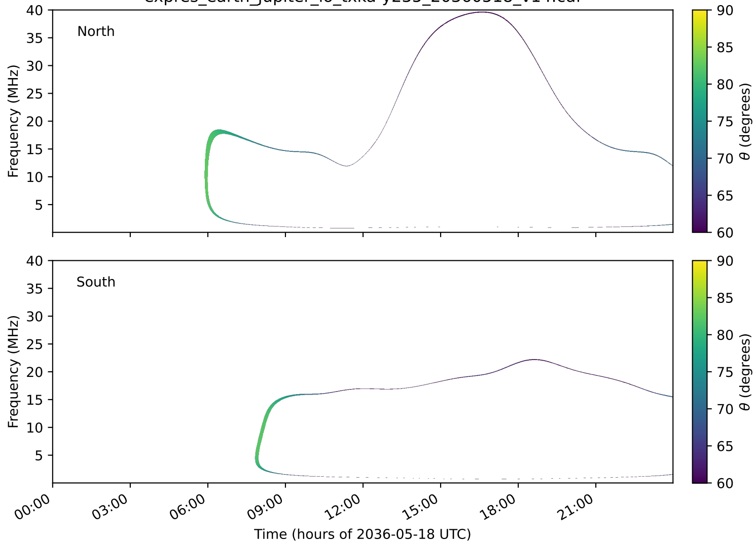
expres_earth_jupiter_io_txka-y235_20360518_v14.cdf
