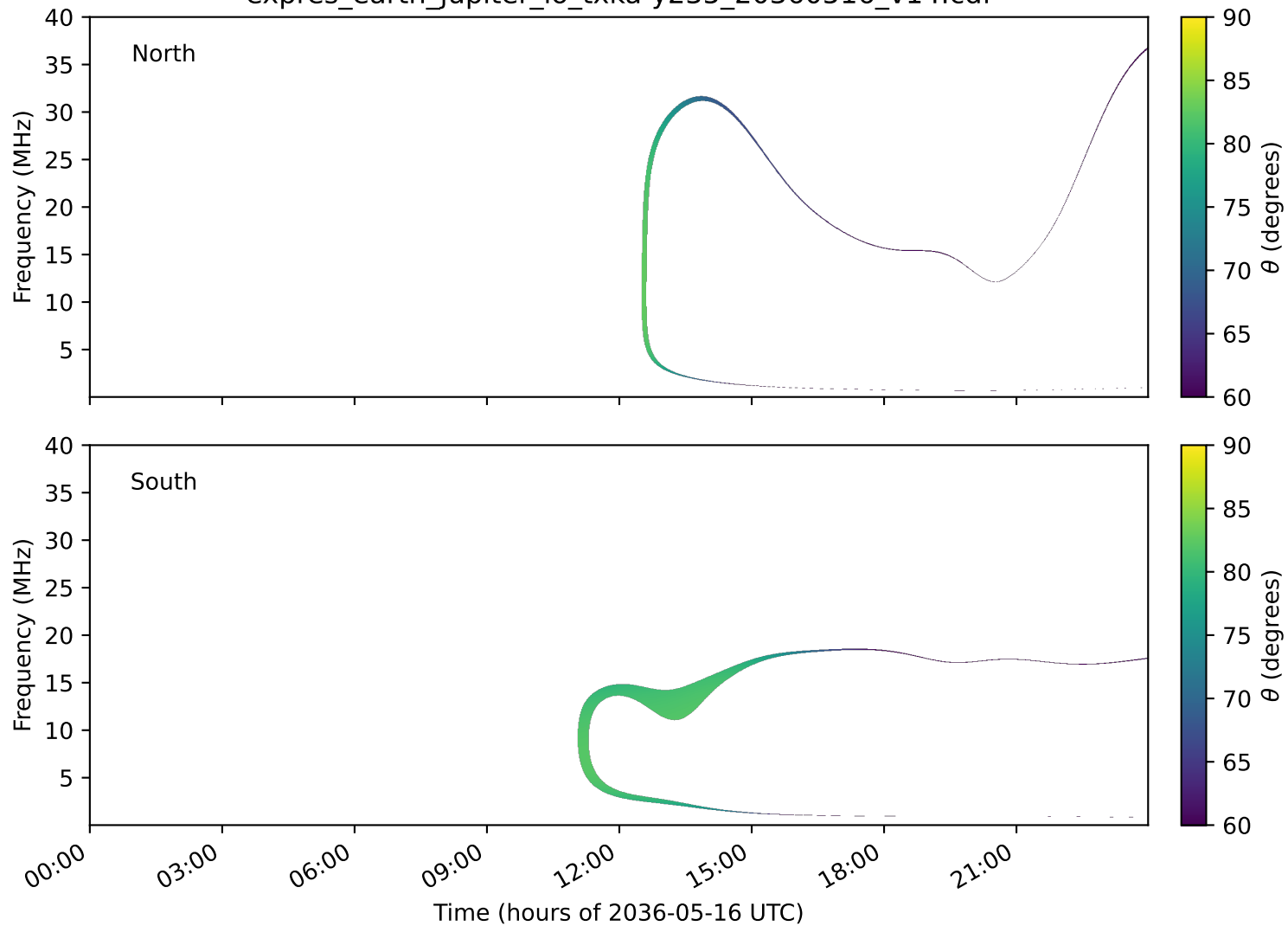
expres_earth_jupiter_io_txka-y235_20360516_v14.cdf
