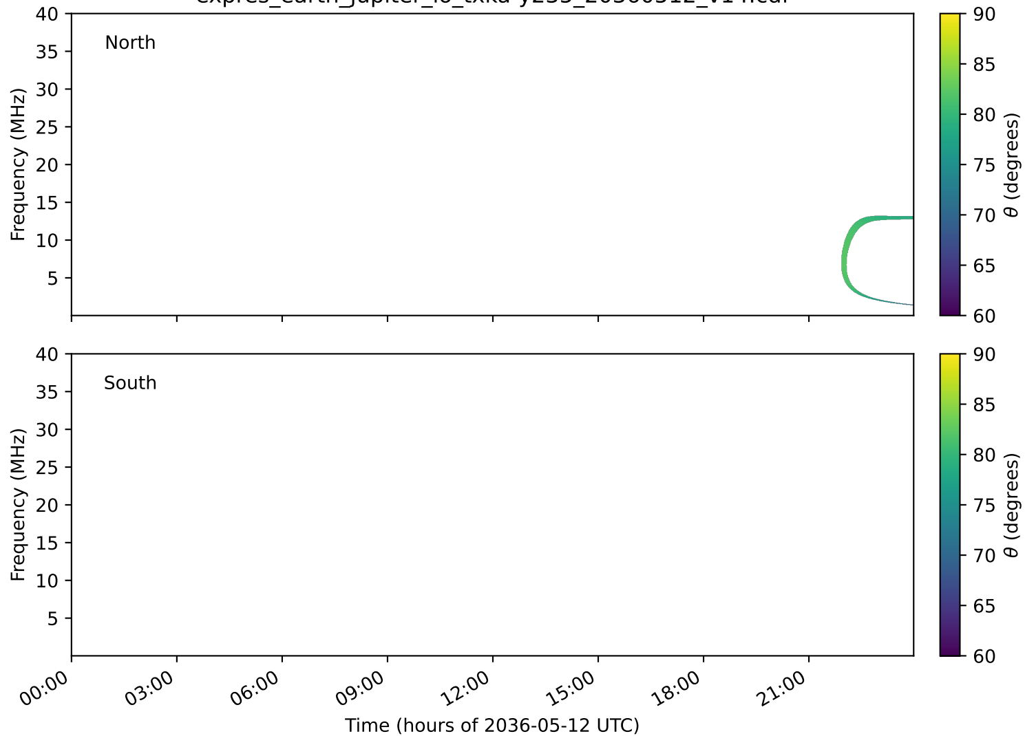
expres_earth_jupiter_io_txka-y235_20360512_v14.cdf
