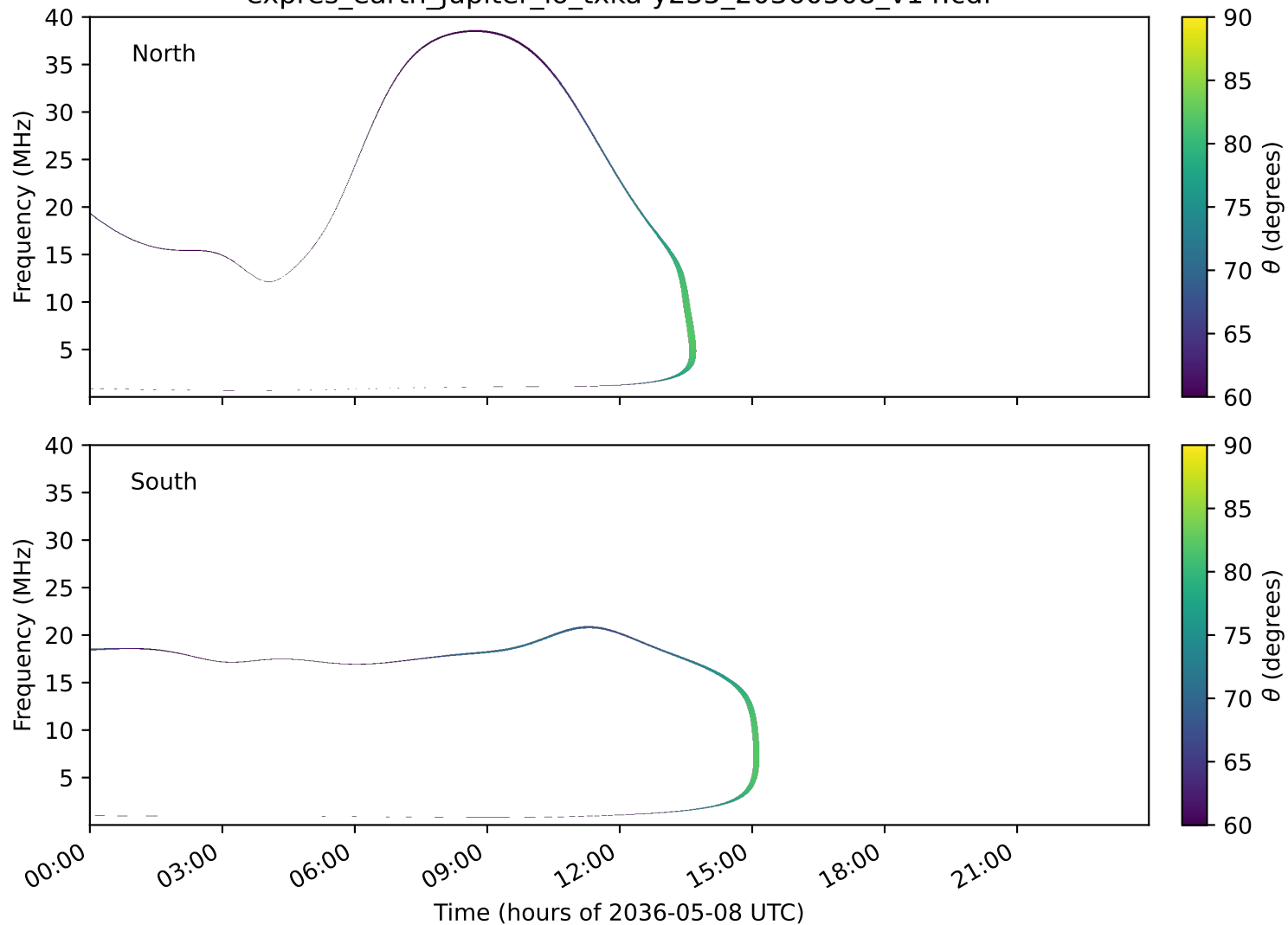
expres_earth_jupiter_io_txka-y235_20360508_v14.cdf
