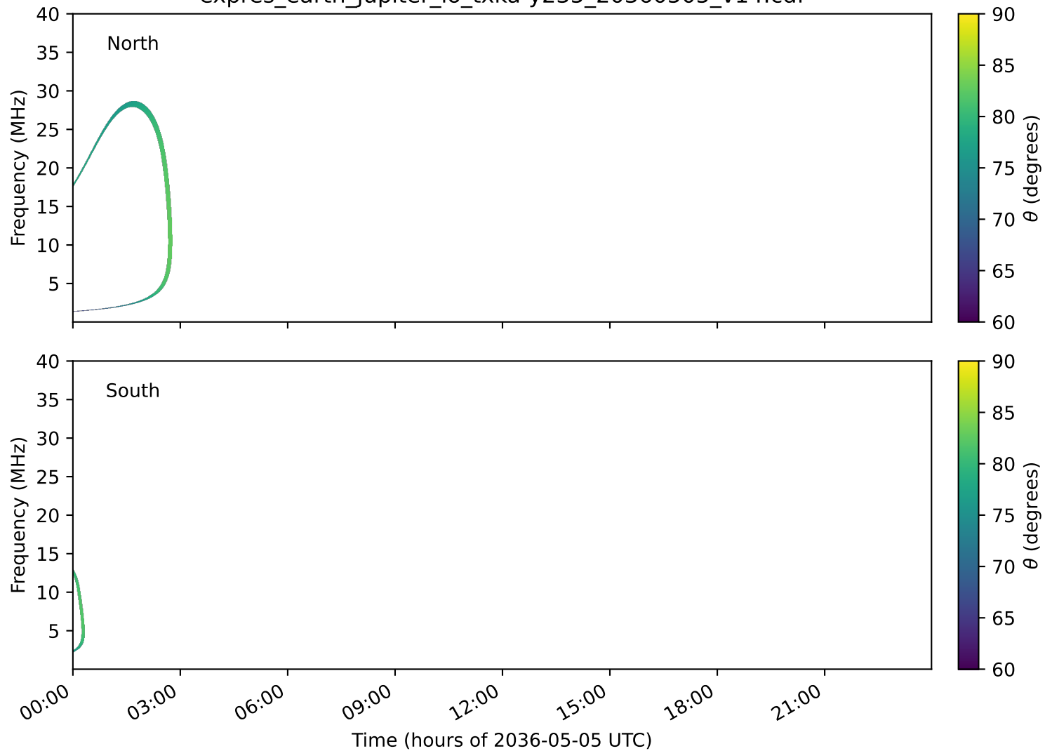
expres_earth_jupiter_io_txka-y235_20360505_v14.cdf
