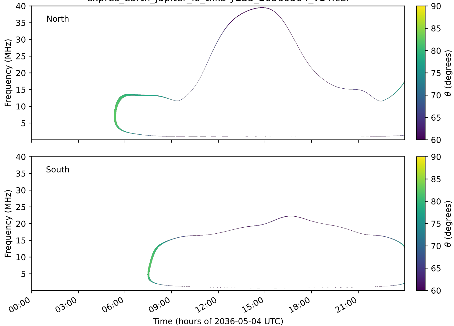
expres_earth_jupiter_io_txka-y235_20360504_v14.cdf
