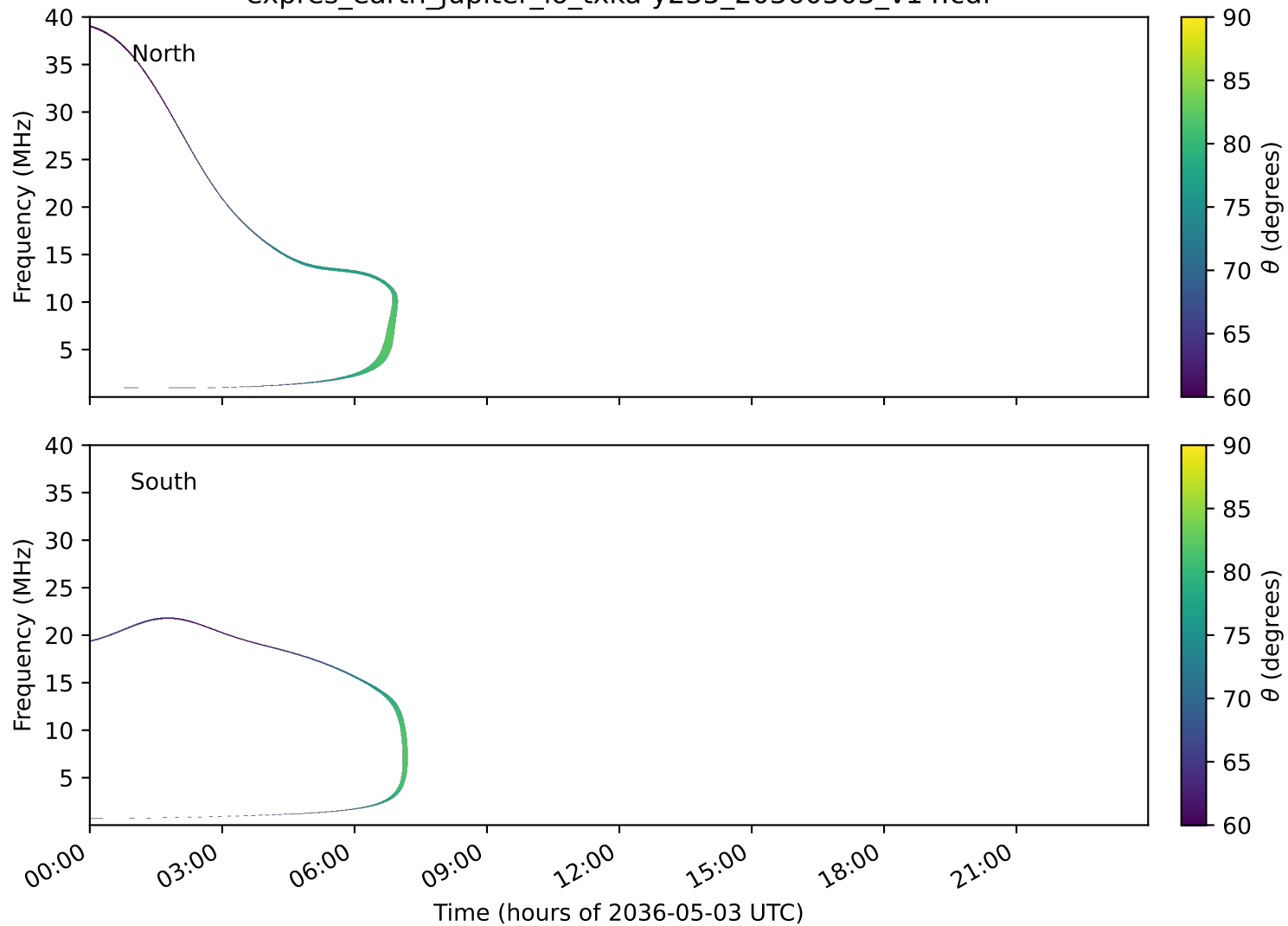
expres_earth_jupiter_io_txka-y235_20360503_v14.cdf
