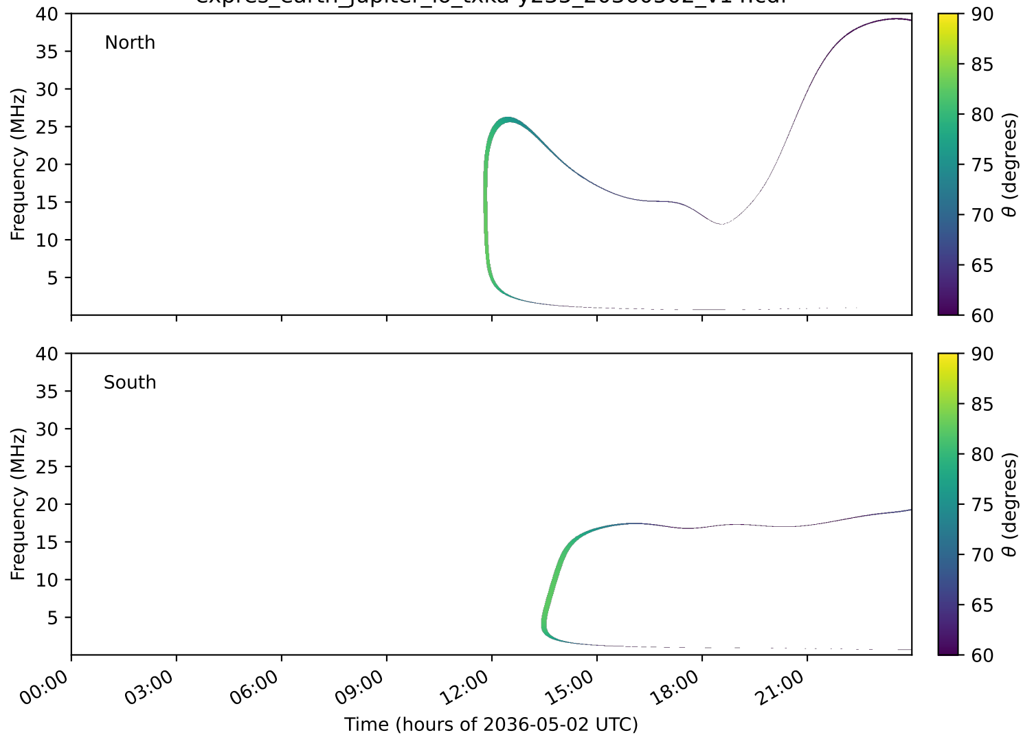
expres_earth_jupiter_io_txka-y235_20360502_v14.cdf
