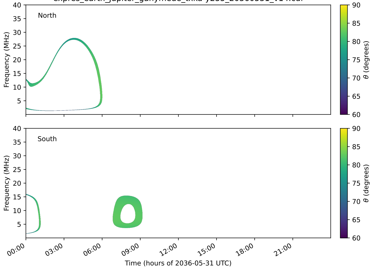
expres_earth_jupiter_ganymede_txka-y235_20360531_v14.cdf
