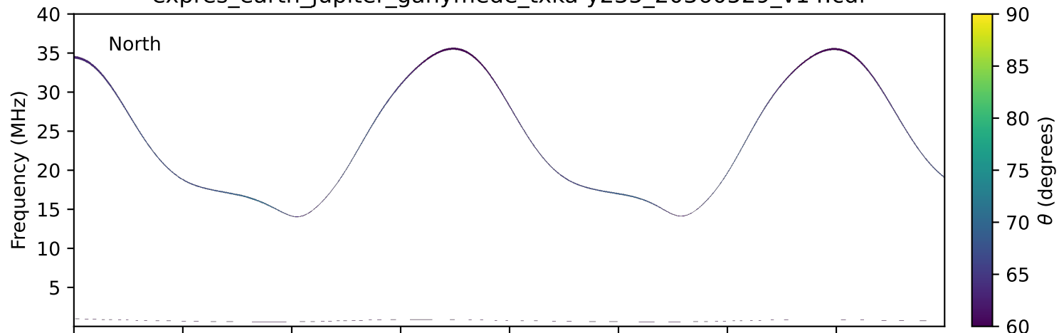
expres_earth_jupiter_ganymede_txka-y235_20360529_v14.cdf
