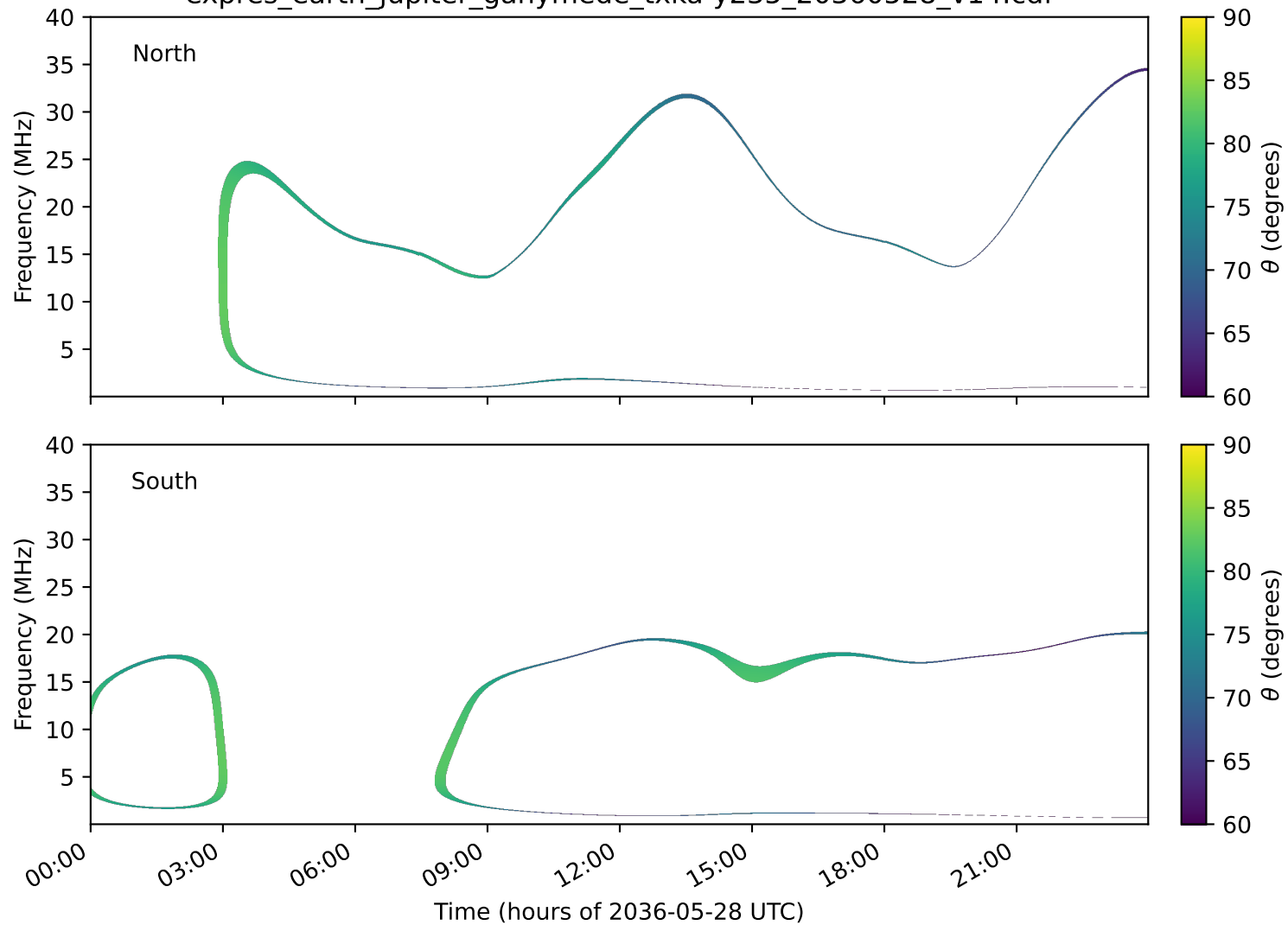
expres_earth_jupiter_ganymede_txka-y235_20360528_v14.cdf
