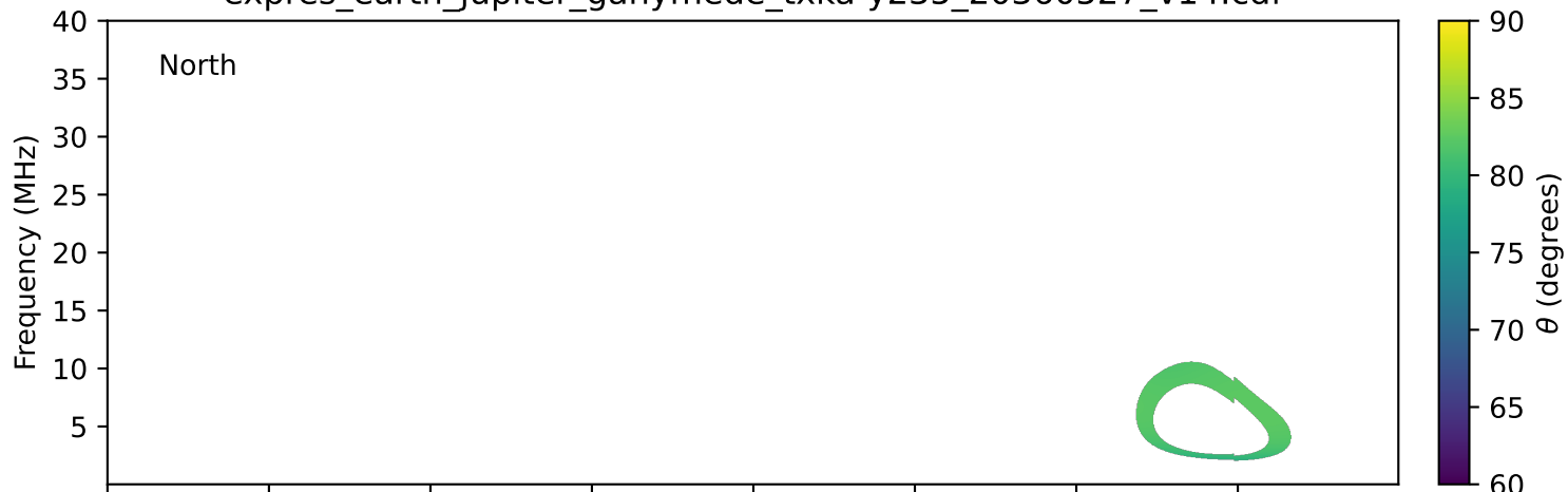
expres_earth_jupiter_ganymede_txka-y235_20360527_v14.cdf
