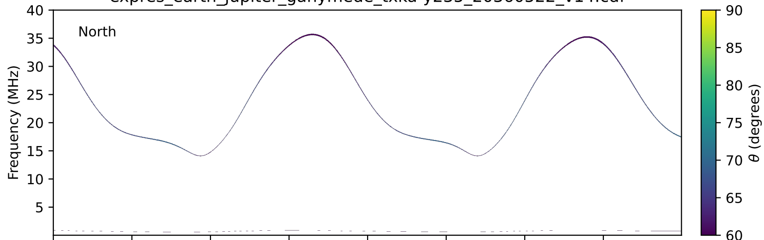
expres_earth_jupiter_ganymede_txka-y235_20360522_v14.cdf
