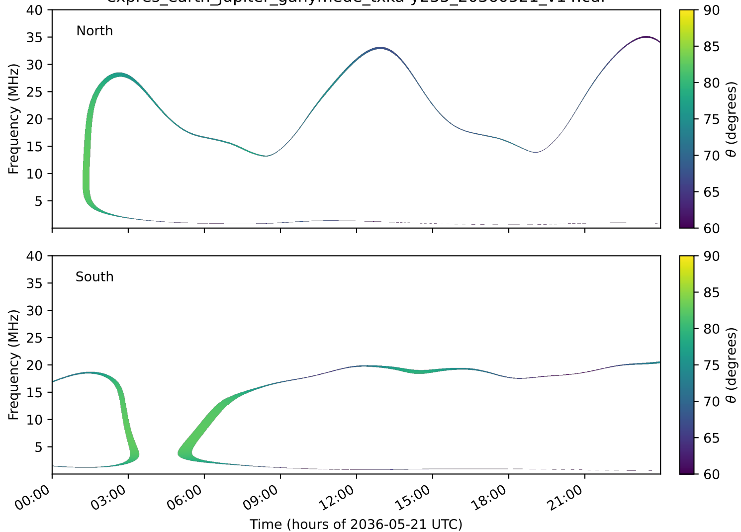
expres_earth_jupiter_ganymede_txka-y235_20360521_v14.cdf
