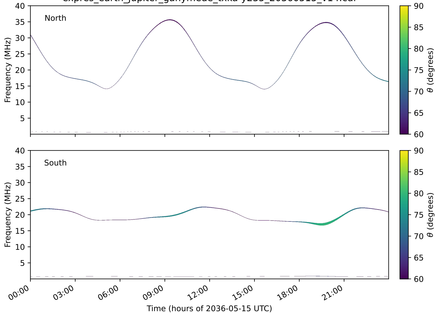
expres_earth_jupiter_ganymede_txka-y235_20360515_v14.cdf
