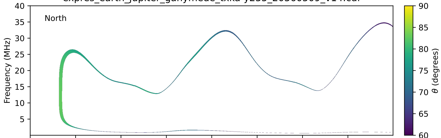
expres_earth_jupiter_ganymede_txka-y235_20360509_v14.cdf
