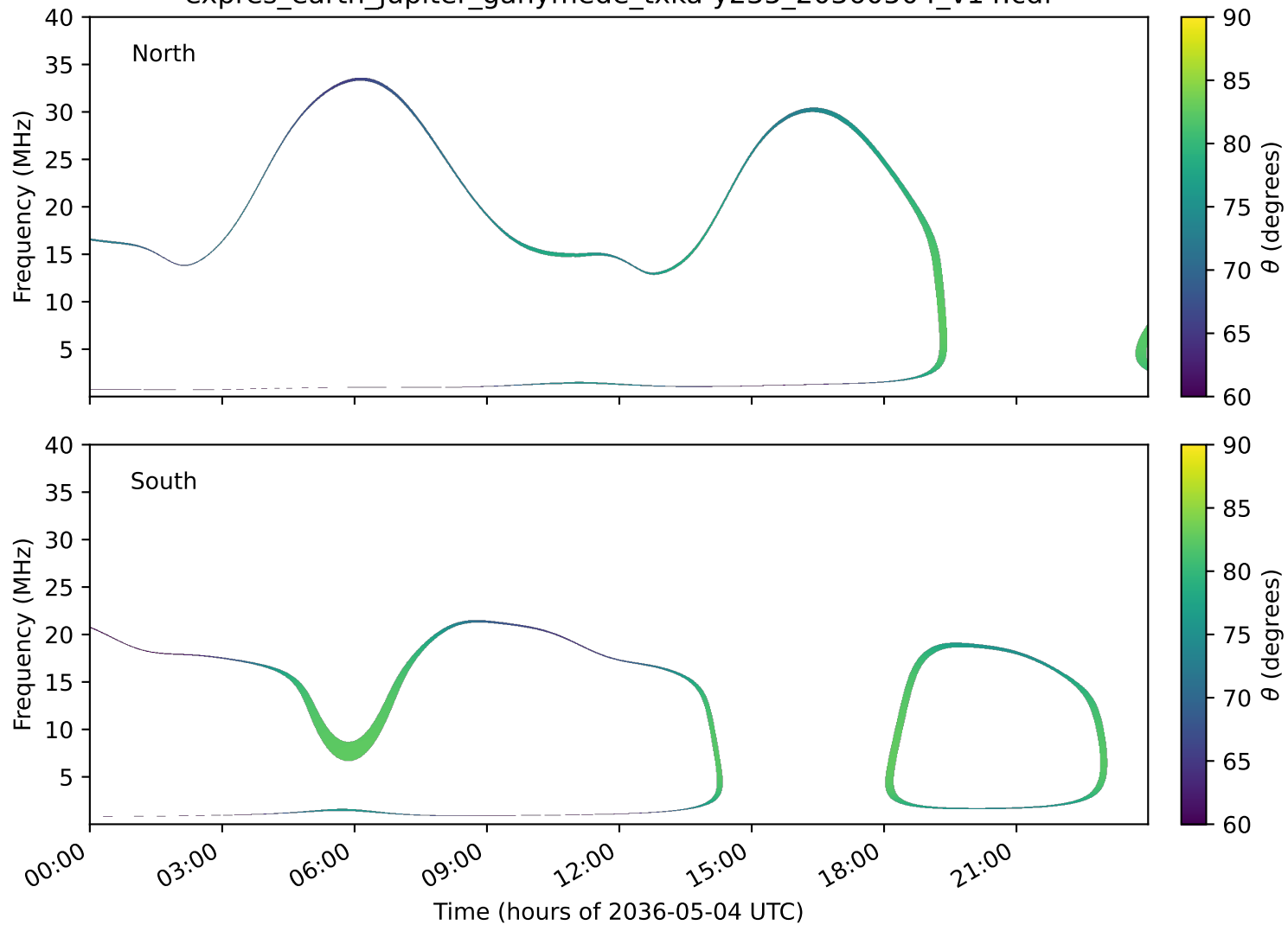
expres_earth_jupiter_ganymede_txka-y235_20360504_v14.cdf
