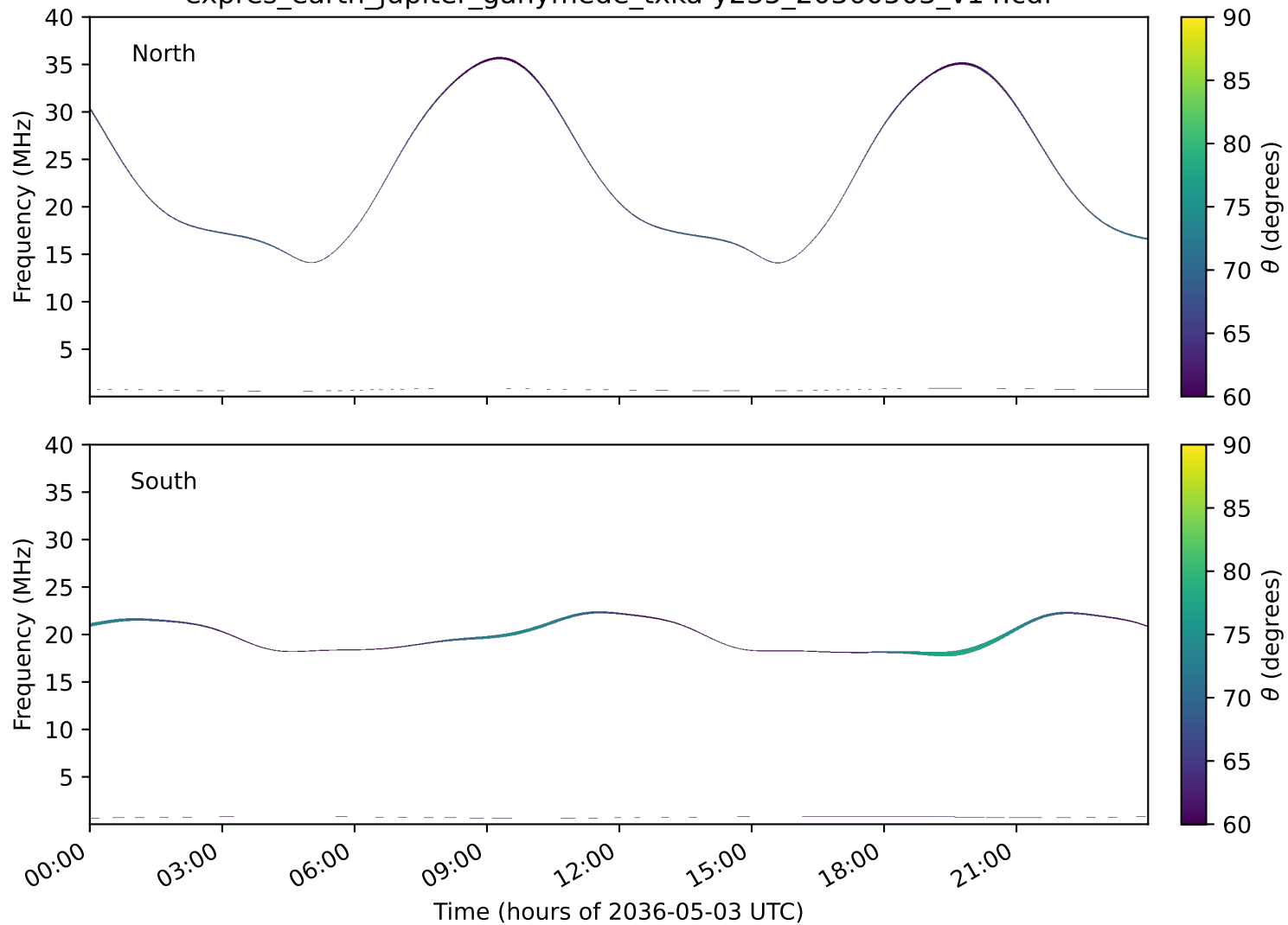
expres_earth_jupiter_ganymede_txka-y235_20360503_v14.cdf
