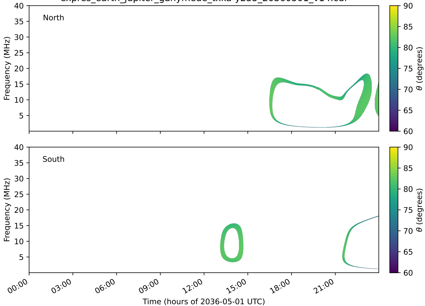
expres_earth_jupiter_ganymede_txka-y235_20360501_v14.cdf
